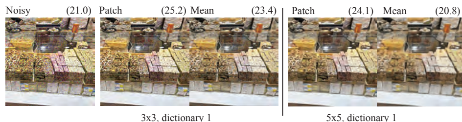
FIGURE 10.12: Approximate nearest neighbor matching yields quite good denoising. On the left , a noisy version of the image of Figure 10.10. Others show reconstructions using the approximate nearest neighbor ( Patch ) or the mean of the query cell ( Mean ) using patches of the size indicated. For these reconstructions, the patches overlap and are averaged (the stride is always 1). In each case, the tree contained 1e7 patches, taken from approximately 200,000 images in the ImageNet test dataset (Section ??), and contains no patches from this image. Image credit: Figure shows my photograph of a sweetshop in Beijing.
