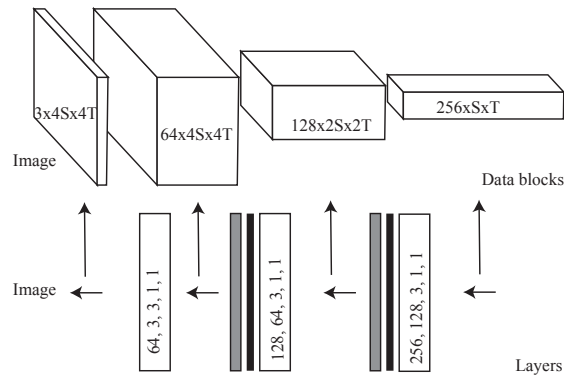
FIGURE 17.3: The architecture of a very simple convolutional decoder, visualized in terms of tensors ( top ), layers ( center - the notation f, d \times x \times y, sN, pM means f filters in the tensor, of spatial extent x \times y , accepting a d dimensional layer, with stride N and padding M ). The receptive field of a decoder is not usually discussed, and I have omitted this here. The thin layers represent ReLU layers. The gray layers represent upsampling by 2 in each dimension. The final pale gray layer could be one of a number of things that are intended to deal with the fact that images have a limited range, including the identity (more details in Section 18.2). I have arranged the filters so that the spatial dimension of the tensor of features leaving the decoder is 4 times that arriving. As is typical, the tensors get spatially bigger but have smaller feature dimension. What goes in is the tensor of codes; you should think of the next tensor as pattern-of-pattern-of-pattern maker; the next as a pattern-of-pattern maker; and so on. Effective convolutional decoders are often significantly deeper and involve further architectural practices, below, but this picture covers the major features for now.
