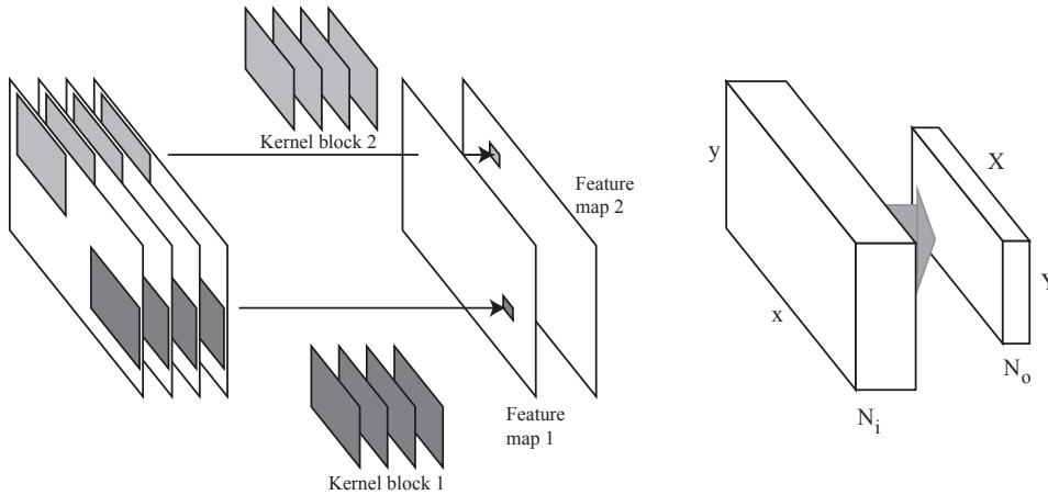
FIGURE 17.1: Multi-channel convolution can be abstracted as a convolutional layer, a linear operation that takes a tensor and produces a tensor. The operation (details in Section 6.1.4) takes a N_i channel tensor (where N_i = 3 for a color image) with dimension N_i \times x \times y and a bank of N_o kernels, each of which is N_i \times d \times d . Apply each filter in the bank to the input tensor to produce one feature channel of dimension 1 \times X \times Y , and add the bias for that channel to each element. Now stack each of these channels, to produce a tensor that is N_o \times X \times Y . Fixed parameters are the input number of features N_i ; the output number of features N_o ; the kernel size d ; the stride s ; and the padding p . I will describe these layers as N_i, N_o, d, s, p in figures that follow. The detailed relationships between x, X and d (etc.) depend on choices about stride, padding and so on exercises .
