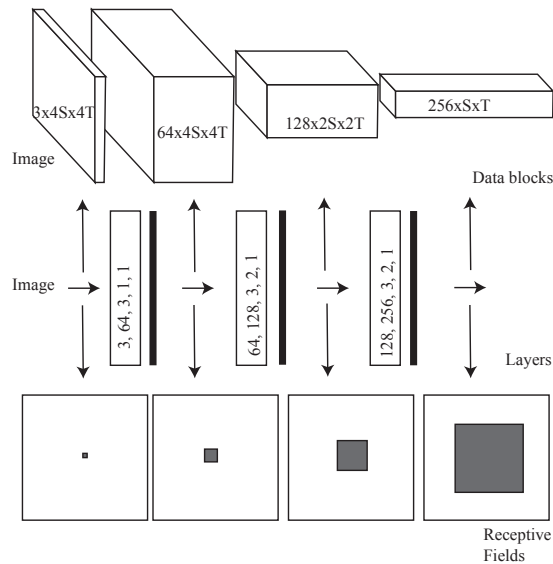
FIGURE 17.2: The architecture of a very simple convolutional encoder, visualized in terms of tensors ( top - the notation f \times x \times y means the tensor has f channels and spatial dimension x \times y ), layers ( center - the notation N_i, N_o, d, s, p means the convolutional layer accepts N_i channels, produces N_o channels, uses d \times d filters, has stride s and padding p ) and receptive fields bottom . The thick lines represent ReLU layers. I have arranged the filters so that the spatial dimension of the tensor of features leaving the encoder is 1/4 of that arriving. As is typical, the tensors get spatially smaller but have larger feature dimension. What goes in is the image; you should think of the next tensor as pattern detector scores; the next as pattern-of-pattern detector scores; and so on. Effective convolutional encoders are often significantly deeper and involve further architectural practices, below.
