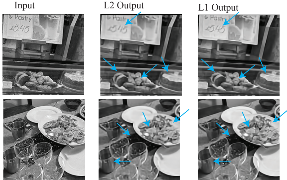
FIGURE 17.7: The L1 loss tends to reduce blur in reconstructed images. Left shows detail tensors from images; center shows the corresponding tensors from an autoencoder trained with SSD loss only; and right shows reconstructions from a simple autencoder trained with an L1 loss only. The effect is small, but it is there (look at the text in the shop window if you're not convinced). Image credit: Images are my photographs of a cheerful dinner table and an enticing shop window.
