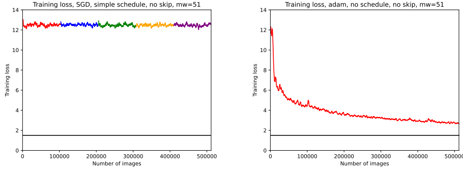
FIGURE 18.9: Adam can improve training behavior for recalcitrant models. Learning curves for the autoencoder with no skip connections using the learning rate schedule in the text left , and with Adam on the right . The curve has been smoothed – you see a moving average of 50 records. This autoencoder just refused to train with SGD, and has trained with Adam, though the loss isn’t wonderful.
