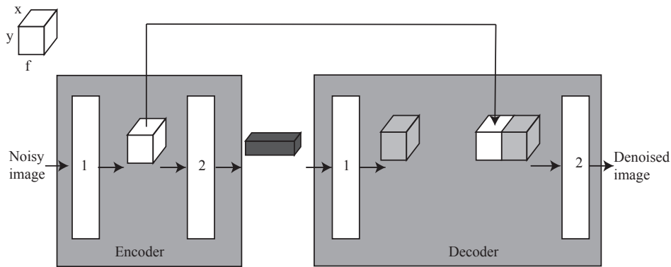
FIGURE 18.1: In a very simple two layer autoencoder with skip connections, the first encoder layer produces a tensor of features (white block; the inset shows the dimensions, two spatial and one feature) which is passed to the second layer. The second layer downsamples to a smaller, deeper tensor (dark gray block). The decoder receives this, passes it through the first decoder layer and upsamples. Arrange the number of filters, etc. to ensure that this tensor has the same spatial extent as the white block (pale gray block). The white block and gray block are stacked along the feature dimension and passed through the second decoder layer. The second decoder layer needs to have more filters, but can now see both short scale features (the white block) and longer scale features (from the dark gray block).
