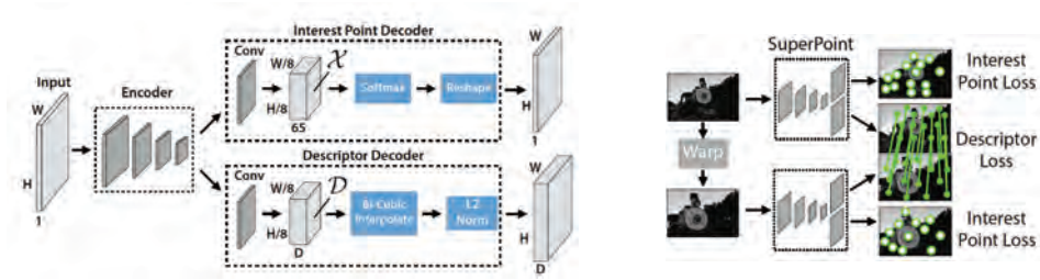
FIGURE 21.7: Attaching a second decoder to SuperPoint makes it possible to produce descriptions for interest points, as well as their locations. On the left , the two decoder architecture. The second decoder produces a d \times (H/8) \times (W/8) block from a H \times W dimensional image. This block is then upsampled using interpolation to form a d \times H \times W block. If the first decoder reports an interest point at i, j in the image, the d values in the second block at location i, j are taken as a vector describing that interest point. These vectors can be trained using a self supervised loss. You know which descriptors should and should not match between a warped version of an image and the original image, yielding the loss. Details in the text. Image credit: Parts of Figure 3 and 2 of “SuperPoint: Self-Supervised Interest Point Detection and Description DeTone et al., 2018.
