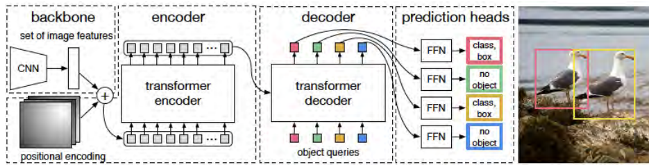
FIGURE 25.9: Image Credit: Part of Figure 1 of End-to-End Object Detection with Transformers Nicolas Carion?, Francisco Massa?, Gabriel Synnaeve, Nicolas Usunier, Alexander Kirillov, and Sergey Zagoruyko
