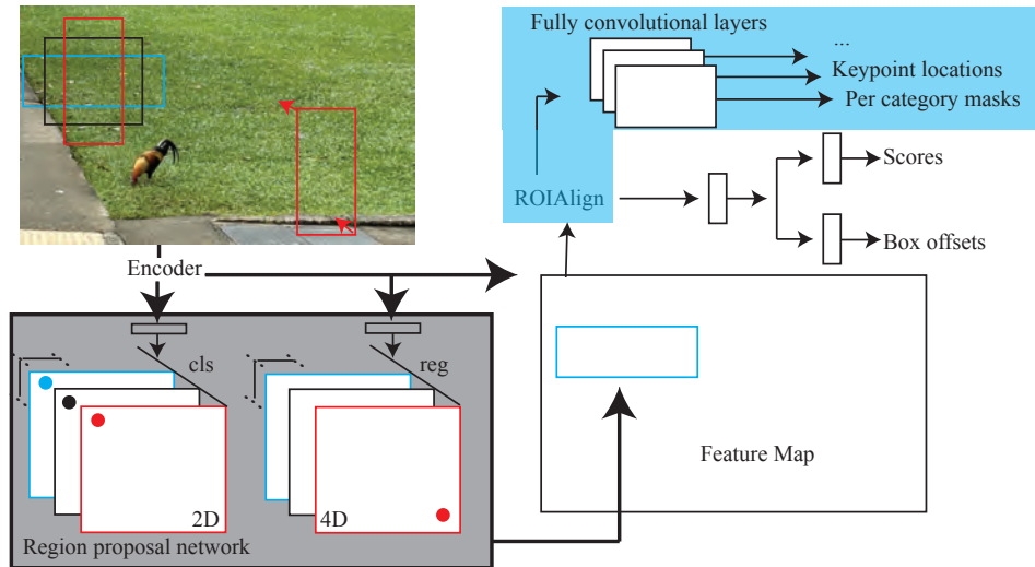
FIGURE 25.4: MaskRCNN involves small but significant modifications to Faster-RCNN which are indicated in the blue boxes (compare to Figure 25.1). ROIPool is replaced with ROIAAlign; and the results are passed through a fully convolutional network to produce a set of fixed size masks, one per category. This procedure can be applied to other predictions as well. I describe keypoint predictions in the text, but the figure leaves room for other possibilities.
