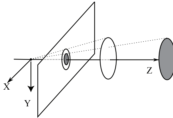
FIGURE 26.4: Two 3D objects of the same size viewed in perspective projection. Division by Z (or, equivalently, similar triangles) means the more distant object appears smaller in the image.
