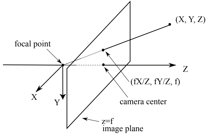
FIGURE 26.2: The usual geometric abstraction of the pinhole model. The box doesn't affect the geometry, and is omitted. The pinhole has been moved to the back of the box, so that the image is no longer inverted. The image is formed on the plane z = f , by convention. Notice the y -axis goes down in the image. This allows me to use a right handed coordinate system and also have z increase as one moves into the image.
