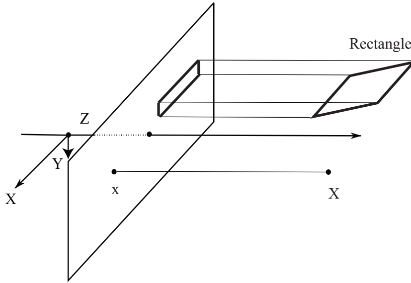
FIGURE 26.8: Scaled orthographic projection with s = 1 is particularly easy to draw (and if s is not 1, one can then rescale the image as required). Here a point \mathbf{X} in 3D projects to a point \mathbf{x} in the image plane by “sliding” down a line perpendicular to the image plane – which is a plane of constant Z , so the line is parallel to the Z axis. In the top right corner, a rectangle is imaged as a foreshortened rectangle. The shortened edges of the rectangle are shortened because they are not parallel to the image plane (exercises).
