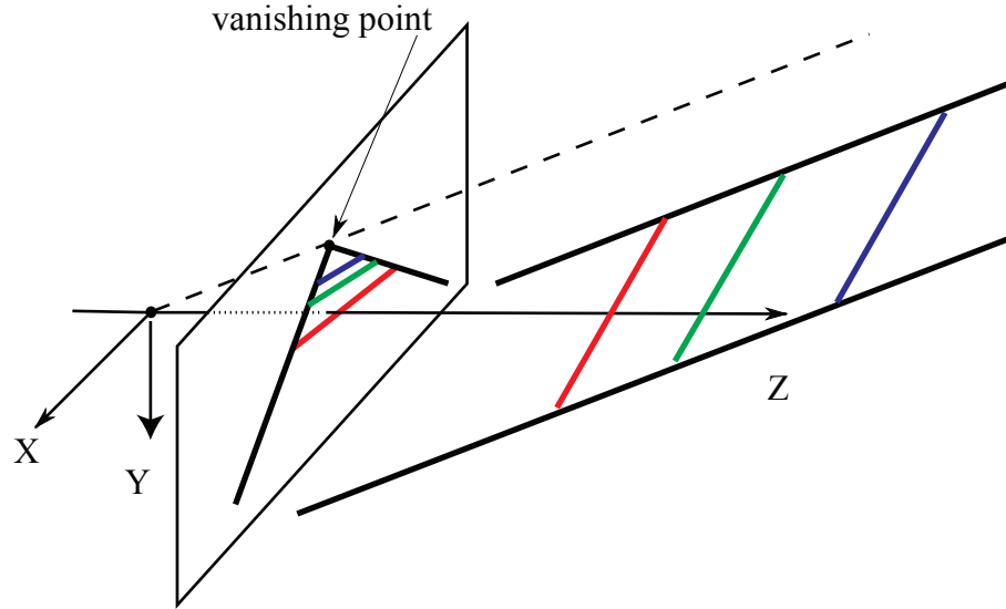
FIGURE 26.6: Here are a different pair of parallel lines from Figure 26.5, with a different vanishing point, and “railway sleepers” still shown. Just as in Figure 26.5, as these sleepers get further away, they get smaller in the image, meaning the projected lines must meet. Just as in Figure 26.5, the vanishing point (the point where they meet) is obtained by intersecting the ray parallel to the lines and through the focal point with the image plane.
