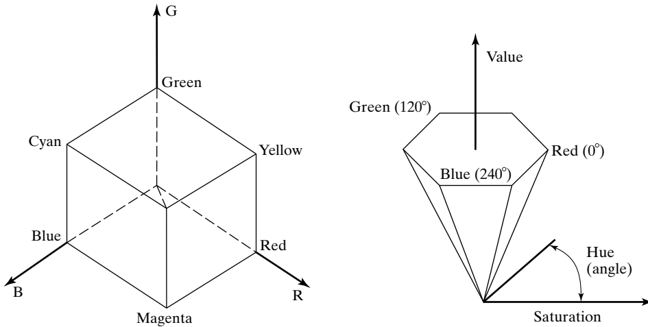
FIGURE 28.13: On the left , we see the RGB cube; this is the space of all colors that can be obtained by combining three primaries (R, G, and B—usually defined by the color response of a monitor) with weights between zero and one. It is common to view this cube along its neutral axis—the axis from the origin to the point (1, 1, 1)—to see a hexagon. This hexagon codes hue (the property that changes as a color is changed from green to red) as an angle, which is intuitively satisfying. On the right , we see a cone obtained from this cross-section, where the distance along a generator of the cone gives the value (or brightness) of the color, the angle around the cone gives the hue, and the distance out gives the saturation of the color.
