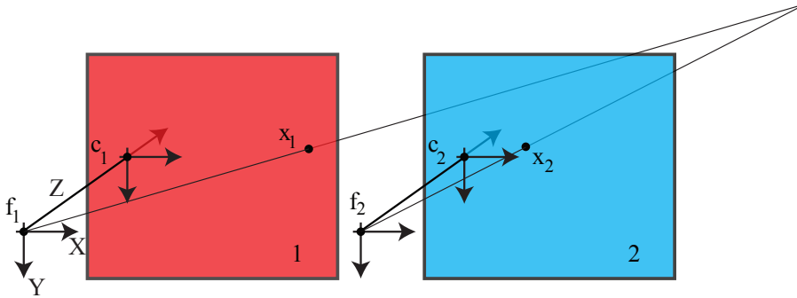
FIGURE 2.8: When two pinhole cameras view a point, the 3D coordinates of the point can be reconstructed from the two images of that point. This applies for almost every configurations of the cameras. It is an elementary exercise in trigonometry ( exercises ) to determine \mathbf{P} from the positions of the two focal points, the locations of the point in the two images, and the distance between the focal points. Considerable work can be required to find appropriate matching points, but the procedures required are now extremely well understood (Chapters 32). One can now buy camera systems that use this approach to report 3D point locations (often known as RGBD cameras). Here we show a specialized camera geometry, chosen to simplify notation. The second camera is translated with respect to the first, along a direction parallel to the image plane. The second camera is a copy of the first camera, so the image planes are parallel. In this geometry, the point being viewed shifts somewhat to the left in the right camera.
