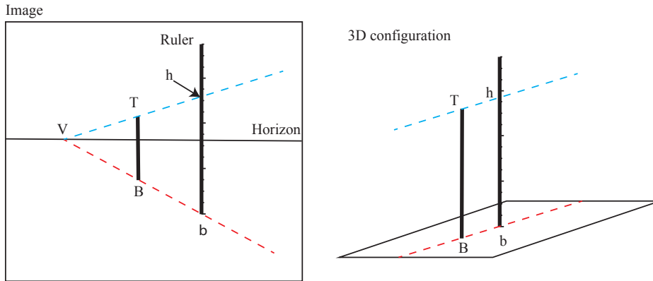
FIGURE 30.3: Left , an image of a ruler and an object, which just both happen to be standing perpendicular to a ground plane. In an uncalibrated image like this, you can measure the height of the object. Construct the line bB (red), and intersect that with the horizon to get the point V . The line from the top of the object T to the true height of the object on the ruler ( h ) is parallel in 3D to bB . In turn, the line Th (blue) must intersect the horizon at V . So if you construct VT , it will intersect the ruler at h yielding the height of the object. Right shows a 3D view; the line Th must be parallel to bB , and so in the image these two lines intersect at the horizon.
