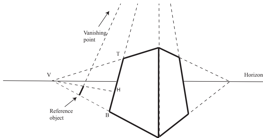
FIGURE 30.7: A building and a person viewed in a more extreme perspective view than that of 30.6. The person has known height, and can act as reference object. The same construction as in that figure yields the height of the building relative to the person.
