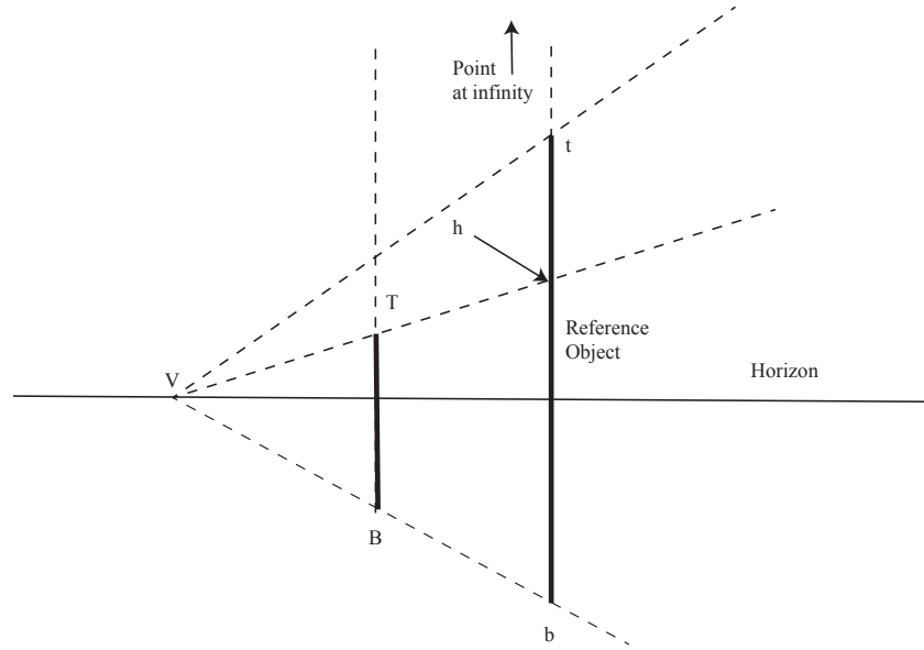
FIGURE 30.6: A perspective camera views a reference object and another object perpendicular to a ground plane. This produces a line segment in the image plane. Constructing appropriate lines in the figure and taking a cross ratio yields the height of the object.
