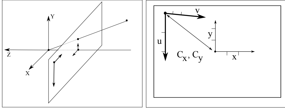
FIGURE 29.5: The camera reports pixel values in pixel coordinates, which are not the same as world coordinates. The camera intrinsics represent the transformation between world coordinates and pixel coordinates. On the left , a camera (as in Figure 26.1), with the camera coordinate system shown in heavy lines. On the right , a more detailed view of the image plane. The camera coordinate axes are marked (u, v) and the image coordinate axes (x, y) . It is hard to determine f from the figure, and we will conflate scaling due to f with scaling resulting from the change to camera coordinates. The camera coordinate system's origin is not at the camera center, so (c_x, c_y) are not zero. I have marked unit steps in the coordinate system with ticks. Notice that the v -axis is not perpendicular to the u -axis (so k - the skew - is not zero). Ticks in the u, v axes are not the same distance apart as ticks on the x, y axes, meaning that s is not one. Furthermore, u ticks are further apart than v ticks, so that a is not one.
