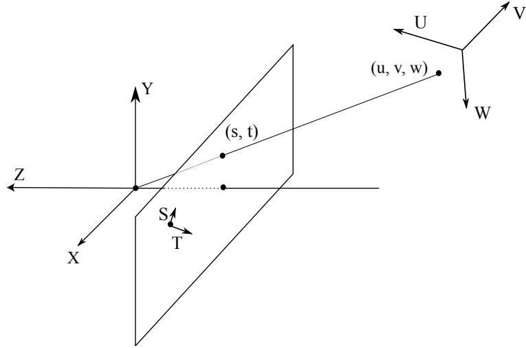
FIGURE 29.4: A perspective camera (in its own coordinate system, given by X , Y and Z axes) views a point in world coordinates (given by (u, v, w) in the UVW coordinate system) and reports its position (s, t) in ST coordinates. The mapping from (u, v, w) to (s, t) consists of a transformation from the UVW coordinate system to the XYZ coordinate system, followed by a perspective projection, followed by a transformation to the ST coordinate system.
