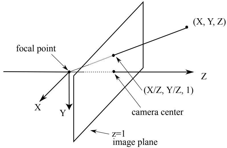
FIGURE 29.3: A canonical pinhole camera is like the usual geometric abstraction, but has image plane z = 1 .
