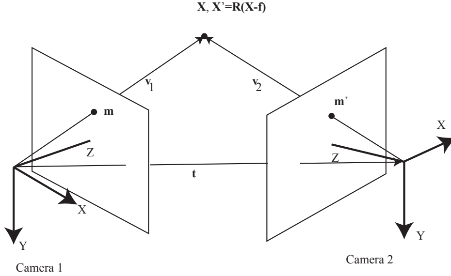
FIGURE 31.3: Camera 1 is in the canonical configuration of Section 29.2 (focal point at the origin, looking down z -axis, image plane at z=1 ). Camera 2 is obtained from camera 1 by a rotation and translation. Each views a point, which is \mathbf{X} in camera 1's coordinate system, \mathbf{X}' = \mathcal{R}(\mathbf{X} - \mathbf{f}) in camera 2's coordinate system. This point projects to \mathbf{m} in camera 1, measured in its coordinate system and \mathbf{m}' in camera 2, measured in its coordinate system. From \mathbf{m} , \mathbf{m}' , \mathcal{R} and \mathbf{f} you can recover \mathbf{X} (or \mathbf{X}' ) using the procedures in the text.
