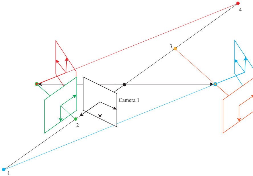
FIGURE 31.4: There are four distinct possible reconstructions for the transformation from camera 1 to camera 2 implied by a known essential matrix. In this figure, camera 1 is at the canonical location; the black point at the center of the figure is camera 1's focal point; and the red, green, blue and orange cameras are the four reconstructions. Notice how red and green are related by a 180^\circ rotation about the translation vector, as are blue and orange. Red and green share a focal point (red with green outline) and blue and orange share a focal point (orange with blue outline). The red-green pair are associated with one sign for the translation estimate (the black arrow), and the blue-orange pair are associated with the other sign. Each reconstruction has a triangulation of a point associated with it. I have marked the point with the same color as the camera 2 reconstruction. Notice how only one triangulation – in this case, the green point – produces a point that lies in front of both camera 1 and the reconstruction. This is the general case. The green camera must be the correct reconstruction.
