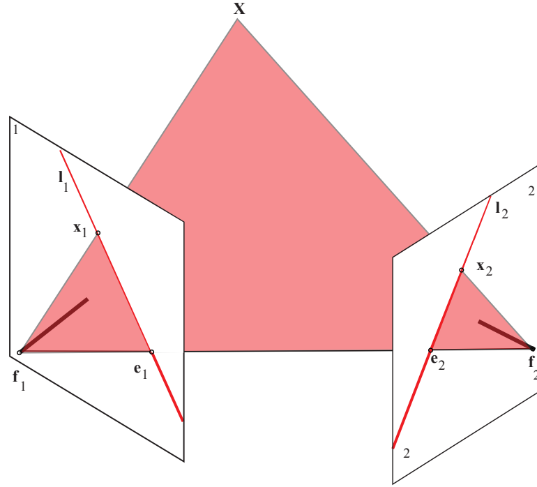
FIGURE 31.1: Two cameras view a point \mathbf{X} in space. The epipoles are formed by the line connecting the focal points ( \mathbf{f}_1 and \mathbf{f}_2 ) of the two perspective cameras (the baseline). This line intersects camera 1's image plane in \mathbf{e}_1 (the epipole in the first image), and camera 2's image plane in \mathbf{e}_2 (the epipole in the second image). As long as the two focal points are distinct, the epipoles are properly defined, although they may appear far outside the image (or even at infinity). The point \mathbf{X} projects to \mathbf{x}_1 in camera 1 and \mathbf{x}_2 in camera 2. The three points \mathbf{f}_1 , \mathbf{f}_2 and \mathbf{X} define a plane in 3D. This plane contains the baseline, and intersects camera 1's image plane in a line ( \mathbf{l}_1 in the figure) that passes through \mathbf{e}_1 and camera 2's image plane in a line ( \mathbf{l}_2 in the figure) that passes through \mathbf{e}_2 .
