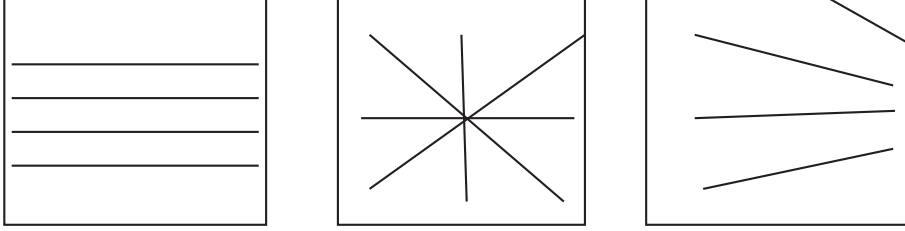
FIGURE 31.2: The epipoles reveal information about how cameras have moved. This is most easily seen by thinking about the epipolar lines. These three examples sketch the underlying intuition, and should be looked at together with Figure 31.1. On the left , the camera has translated parallel to the image plane; center , the camera has moved perpendicular to the image plane; and right , the camera has translated parallel to the image plane then rotated slightly. You should check each case carefully.
