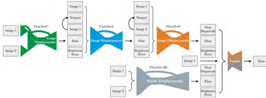
FIGURE 36.2: FlowNet2 obtains significant improvements by composing multiple Flownets. Compute a flow estimate with a flownet; now warp the second image to produce \mathcal{W} (which would be frame 1 if you had the flow right). The magnitude of the residual between frame 1 and the warped version of frame 2 identifies errors in the flow. Provide this error, \mathcal{I}_1 and \mathcal{W} to a version of flownet adjusted to accept the extra frames. This produces a revised flow. You can stack these revised versions as required (two seems to be enough). The resulting network is good at estimating large flows. Now build yet another flownet, allowing quite small displacements only. You now have two estimates of flow, so construct a fusion network that accepts the flow estimates and produces a final fused estimate. Show this network \mathcal{I}_1 , the flow fields, the flow magnitudes, and the brightness errors (Figure ??). Image credit: Figure 2 of FlowNet 2.0: Evolution of Optical Flow Estimation with Deep Networks, by E. Ilg, N. Mayer, T. Saikia, M. Keuper, A. Dosovitskiy and T. Brox.
