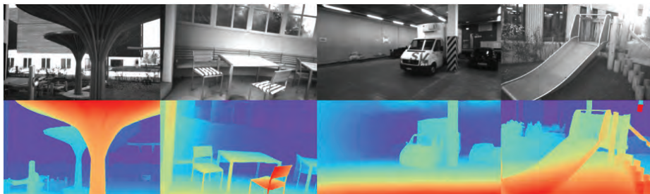
FIGURE 36.10: RAFT-Stereo produces very strong disparity estimates. Top row shows frames from the ETH3D stereo dataset and bottom row shows recovered disparities. Notice that (a) there are precise boundaries in the right place; (b) there is very little spatial noise; and (c) there are sensible disparity estimates in regions that should be very hard to match. For example, matching must be very hard on near featureless surfaces, but the table in column 2, floor in column 3, and slide in column 5 are well reconstructed. Image credit: Figure 4 of RAFT-Stereo: Multilevel Recurrent Field Transforms for Stereo Matching, by L. Lipson, Z. Teed and J. Deng.
