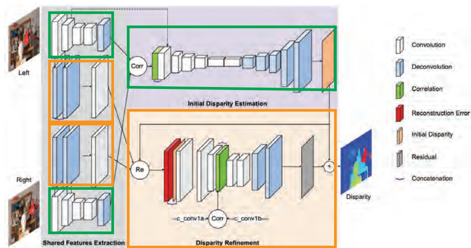
FIGURE 36.4: Liang et al.[1] estimate stereo disparity using two coupled networks. The first, outlined in green , produces a disparity estimate by: encoding left and right images, computing a cost-volume, then decoding that with 3D convolution and soft argmin (as in Section ??). This results in a disparity estimate (the orange block on the right ). A second network, outlined in orange , refines this estimate using procedures in the main text. Image credit: Figure 2 of Z. Liang et al., "Stereo Matching Using Multi-Level Cost Volume and Multi-Scale Feature Constancy," in IEEE Transactions on Pattern Analysis and Machine Intelligence , vol. 43, no. 1, pp. 300-315, 1 Jan. 2021
