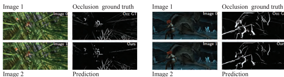
FIGURE 36.16: A variant of FlowNet2 can predict occlusions as well as flow or disparity. For each of these pairs of frames from SINTEL, the figure shows the ground truth occlusions (known because SINTEL is rendered from 3D models; above ) and the predicted occlusions ( below ). Note how fine occlusions are predicted very accurately. Image credit Part of Figure 2 of “Occlusions, Motion and Depth Boundaries with a Generic Network for Disparity, Optical Flow or Scene Flow Estimation”, by E. Ilg, T. Saikia, M. Keuper, and T. Brox
