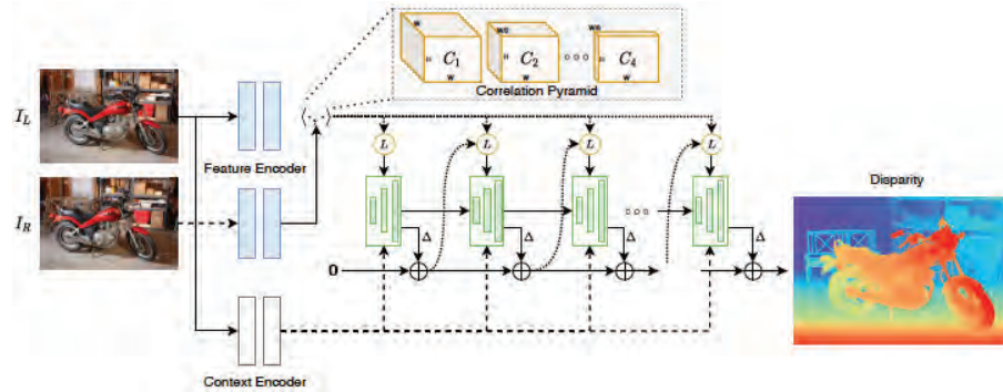
FIGURE 36.9: RAFT-Stereo follows RAFT (compare this figure with Figure 36.6). Encode frame 1 and frame 2 to produce a feature representation, then computes a cost-volume. Pool and subsample this to form representations at coarser and coarser scales. An incremental procedure then starts with zero disparity, and repeatedly updates the disparity using the previous disparity estimate, a context feature, and a readout from the multi-scale representation. Image credit: Figure 1 of RAFT-Stereo: Multilevel Recurrent Field Transforms for Stereo Matching, by L. Lipson, Z. Teed and J. Deng.
