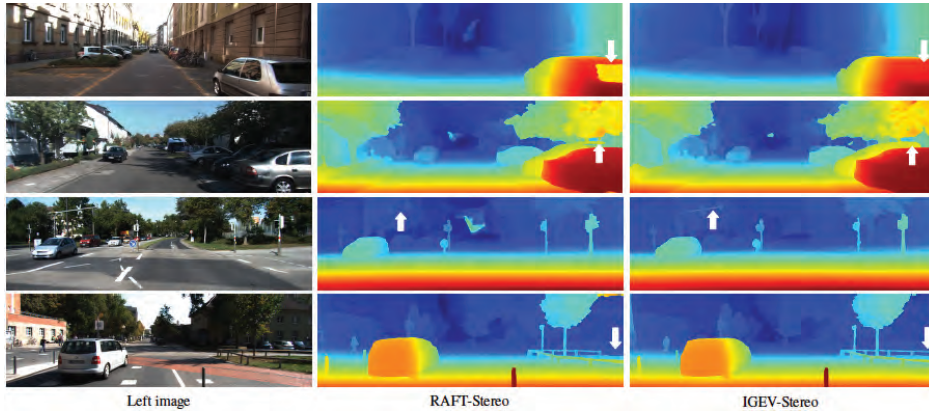
FIGURE 36.12: IGEV disparities (right) compared with RAFT-Stereo disparities (center), showing important small improvements in detailed reconstruction. The white arrows point out details. Note the improved rear windscreen in the top row; the improvement in the traffic light gantry ( center row); and the improvement in the rails in the bottom row. Here Image credit: Figure 4 of Iterative Geometry Encoding Volume for Stereo Matching, by G. Xu, X. Wang, X. Ding and X. Yang
