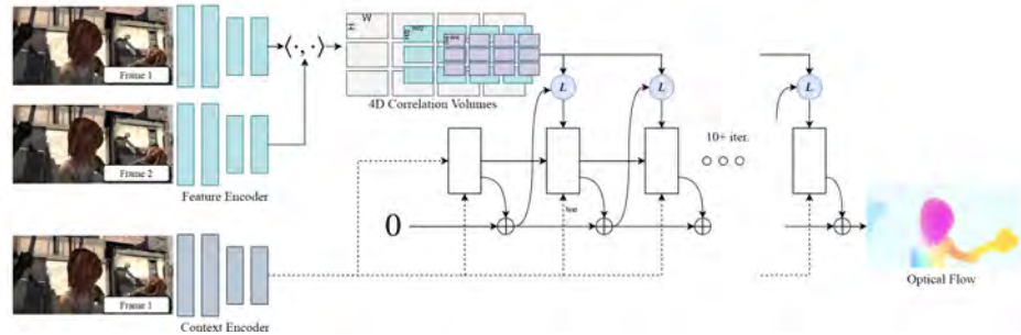
FIGURE 36.6: RAFT encodes frame 1 and frame 2 to produce a feature representation, then computes an inner product between features for every pair of locations in frame 1 and frame 2. This volume of inner products is then pooled and subsampled to form representations at coarser and coarser scales. Pooling is done so you can tell where a specific pixel in frame 1, represented in the original resolution, went to in frame 2 at various resolutions. The result is a representation of flow at multiple levels of precision. An incremental procedure then starts with zero flow, and repeatedly updates the flow using the previous flow estimate, a context feature, and a readout from the multi-scale representation. Image credit: Figure 1 of RAFT: Recurrent All-Pairs Field Transforms for Optical Flow by Z. Teed and J. Deng.
