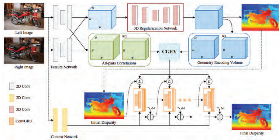
FIGURE 36.11: The architecture of IGEV stereo (compare with Figure 36.10). IGEV improves over RAFT-Stereo by computing an estimate of 3D geometry (top left – compare single image depth maps), encoding that, and using it during the iterative reestimation procedure. Image credit: Figure 3 of Iterative Geometry Encoding Volume for Stereo Matching, by G. Xu, X. Wang, X. Ding and X. Yang
