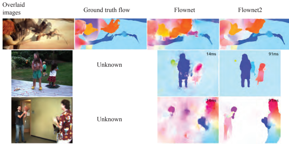
FIGURE 36.3: Flownet2 predictions are a significant improvement over Flownet predictions. The top row shows qualitative results on an example image from the SINTEL dataset (Section 36.2). The overlaid image is an average of first and second frame, so you can identify flows by “ghosting” of edges. The direction of a flow vector is shown by hue (what changes from red to yellow to green to purple) and the magnitude by saturation (very small vectors are white, longer are pale colors, longest have intense colors). Notice how much more detail there is in Flownet2 estimates. SINTEL is rendered, so the ground truth flow is known, and you can compare. The bottom rows show flow predictions for real image pairs, where the ground truth is unknown. Again, Flownet2 produces much more detailed flow fields; they should look like highly plausible flow estimates to you. Image credit: Parts of Figure 6 and 7 of FlowNet 2.0: Evolution of Optical Flow Estimation with Deep Networks , by E. Ilg, N. Mayer, T. Saikia, M. Keuper, A. Dosovitskiy and T. Brox.
