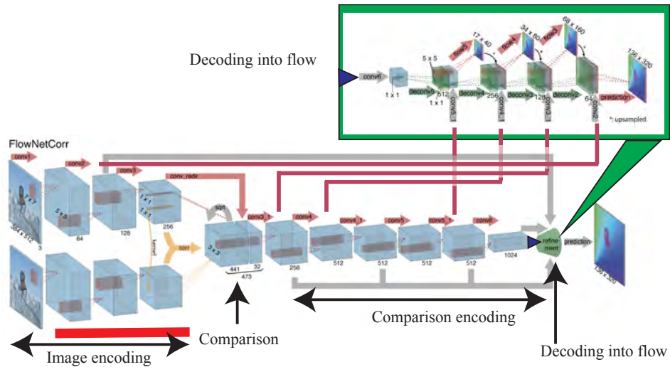
FIGURE 36.1: The overall architecture of FlowNet, a regression based optic flow predictor ([1]). The frames pass through an image encoder; the results are compared (details in text), and the comparison further encoded. Finally, the result is decoded into a flow field, using skip connections from the comparison encoder and from the first frame encoder. Image credit: Figure 2 of FlowNet: Learning Optical Flow with Convolutional Networks by P. Fischer, A. Dosvitskiy, E. Ilg, P. Hausser, C. Hazirbas, V. Golkov, P. van der Smag, D. Cremers, and T. Brox
