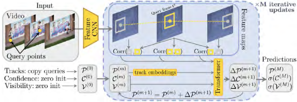
FIGURE 40.15: CoTracker3 trains a transformer to update estimates of position ( P ), confidence ( C ), and visibility ( V ) for a query point at each frame. The transformer accepts (\mathcal{P}^i, \mathcal{C}^i, \mathcal{V}^i) and image features for frame i , and produces an update to each to form these estimates for the next frame. The transformer is trained with labelled data, including synthetic data sets constructed with known point correspondences, and real datasets labelled by “teacher” tracker models. Figure constructed using parts of Figure 2 of “CoTracker3: Simpler and Better Point Tracking by Pseudo-Labeling Real Videos”, Karaev et al, 2024
