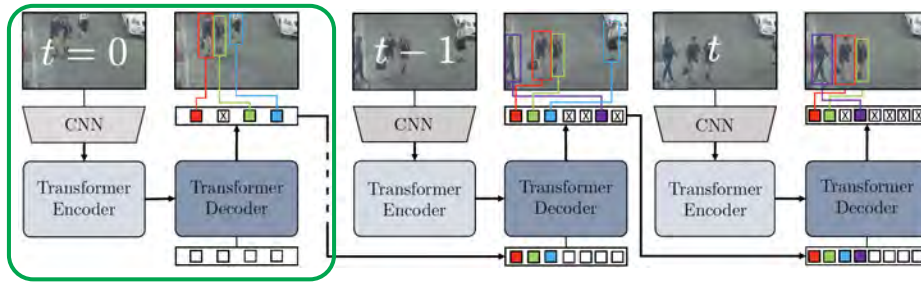
FIGURE 40.8: Detr uses a transformer to combine image tokens and object query tokens into detection tokens, that are then decoded into either “no object” or a box location and category scores (green box). In Trackformer [], the detection tokens are adjusted and passed on as query tokens. These are combined with tokens for the next frame to produce detection tokens, and so on. Image credit: Figure 1 of “Tracking without bells and whistles’TrackFormer: Multi-Object Tracking with Transformers”, Meinhardt et al, 2021
