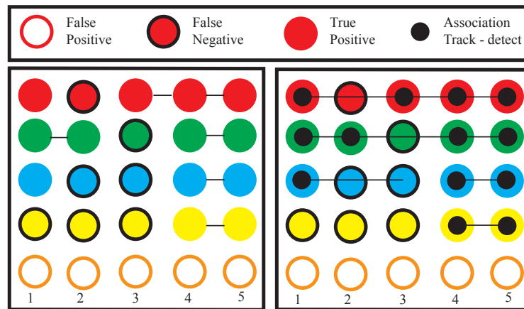
FIGURE 40.2: The simplest tracking by detection procedure breaks up tracks when objects are occluded. Allowing abstract tracks solves this problem. Each column is a frame; each colored circle is a detector response. Full colored circles are detector responses that correctly identify an object. Colored circles with a black boundary are false negatives – the object is in the frame, but the detector didn’t respond to it. Each object is represented by a consistent color. Empty circles with colored boundaries are false positives – there is no underlying object. For these, the color has no particular meaning because there is no underlying object. The simplest procedure ( left ) just links detector responses to the next frame. There is no way to represent an object that is missed for a frame, so the tracks break up. If you allow abstract tracks ( right ), tracks can be kept even if a measurement is missing. An association between a track and a detector response is given by a small dark circle. There isn’t one on a false negative, because there is no measurement to link the track to. For this figure, the track is allowed to go one frame without a measurement, and is then reaped. A new measurement results in a new track being created ( blue; yellow ).
