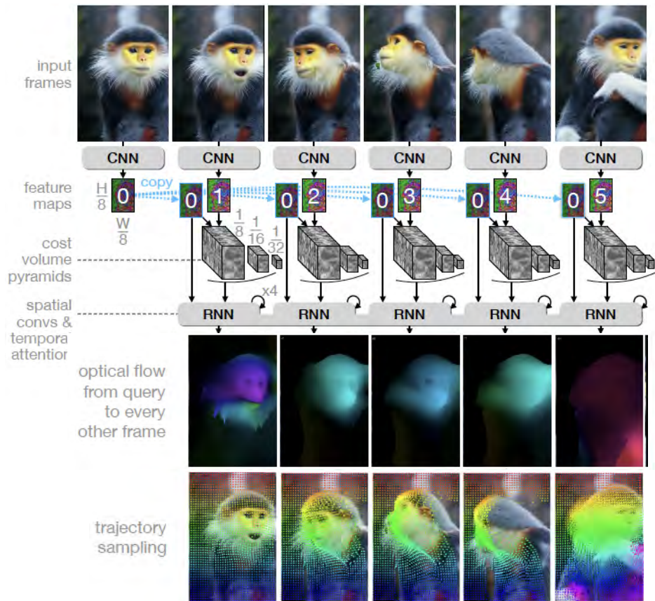
FIGURE 40.16: Figure constructed using parts of Figure 2 of “AllTracker: Efficient Dense Point Tracking at High Resolution”, Harley et al, 202X
