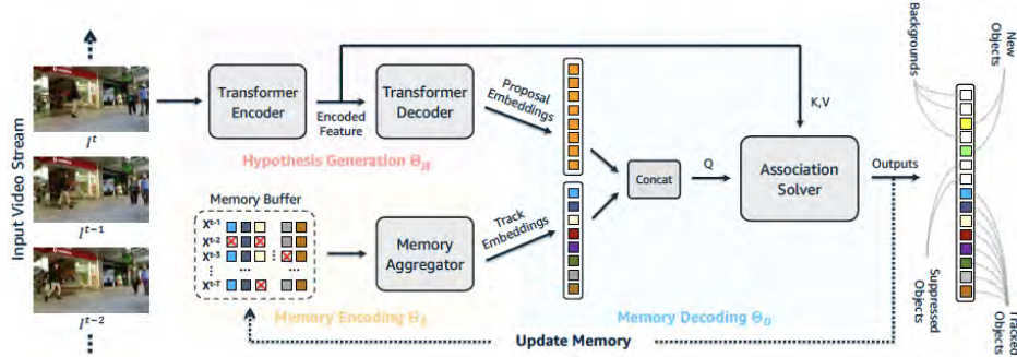
FIGURE 40.10: MeMOT maintains a memory buffer containing image embeddings associated with tracks seen in the past. This memory buffer is used to support allocating object windows to tracks and to identify instances that have not been seen before. A transformer encoder/decoder produces a set of tokens representing the possible objects in the image (as in DeTR, Section 21.3). These tokens are concatenated with a set of tokens from memory. The resulting set is decoded to identify instances that should be attached to tracks and those that are new objects. Some image tokens that represent objects are suppressed, because they are explained by memory tokens. Others are background, or novel instances. Tokens that represent objects are then used to update the memory. Image credit: Figure 2 of “MeMOT: Multi-Object Tracking with Memory”, Cai et al, 2023.
