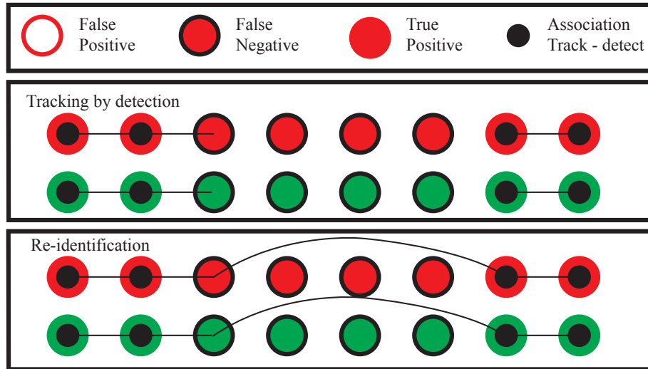
FIGURE 40.3: If an object is occluded for long enough, procedure 40.1 will break up the track. Reidentification creates links between object detector responses where there is strong evidence the object is the same.
