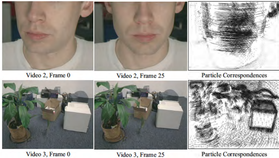
FIGURE 40.13: You can build relatively dense, relatively long term, tracked representations of points in images using optical flow. Choose a collection of points in the first frame, then allow points to flow along the flow field. Maintain the representation at each frame using two procedures. Reap points if the flow is unreliable, and add points in regions where the point density is too low. The result is a collection of short to medium time point tracks that are relatively dense in the image. Left column shows first frame of two sequences; center column shows late frames in those sequences; right column shows the resulting point tracks. Some tracks survive for long periods and others for shorter periods. The points have fairly high density. Figure constructed using parts of Figure 6 of “Particle Video: Long-Range Motion Estimation using Point Trajectories”, Sand and Teller, 06.
