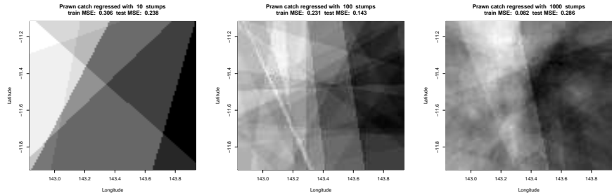
FIGURE 16.6: Visualizations of the predictor for the prawn data of worked example 16.4. Mid-grey is zero; white is positive (and so any shade in the range mid-grey to white predicts a score greater than the median); black is negative (and so any shade in the range mid-grey to black predicts a score less than the median). The predictor formed by one stump cuts the region into two halves with a line; on one side of the line, it takes one constant value, and on the other, it takes a different constant value. Adding many of these together results in a function that is constant in each cell of an arrangement of lines. Predictors that use more stumps produce more complicated functions of this form, with improvements in training error and some improvement in test error (Figure 16.6).
