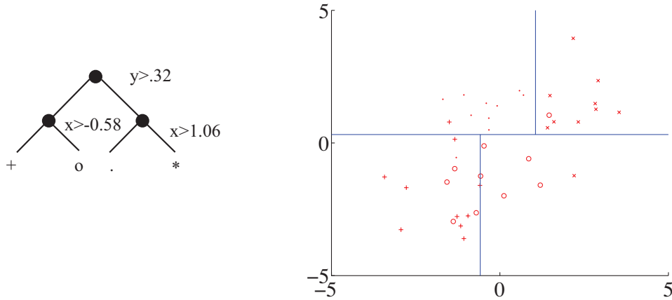
FIGURE 1.5: A straightforward decision tree, illustrated in two ways. On the left , I have given the rules at each split; on the right , I have shown the data points in two dimensions, and the structure that the tree produces in the feature space.
