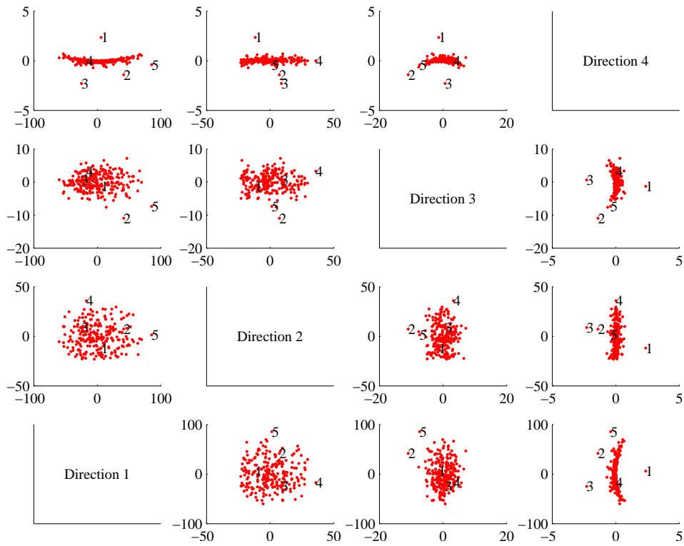
FIGURE 2.9: A panel plot of the bodyfat dataset of figure 2.4, now rotated so that the covariance between all pairs of distinct dimensions is zero. Now we do not know names for the directions — they’re linear combinations of the original variables. I have scaled the axes so you can see details; notice that the blob is a little curved, and there are several data points that seem to lie some way away from the blob, which I have numbered.
