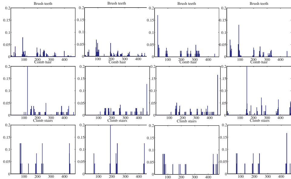
FIGURE 3.15: Histograms of cluster centers for the accelerometer dataset, for different activities. You should notice that (a) these histograms look somewhat similar for different actors performing the same activity and (b) these histograms look somewhat different for different activities.
