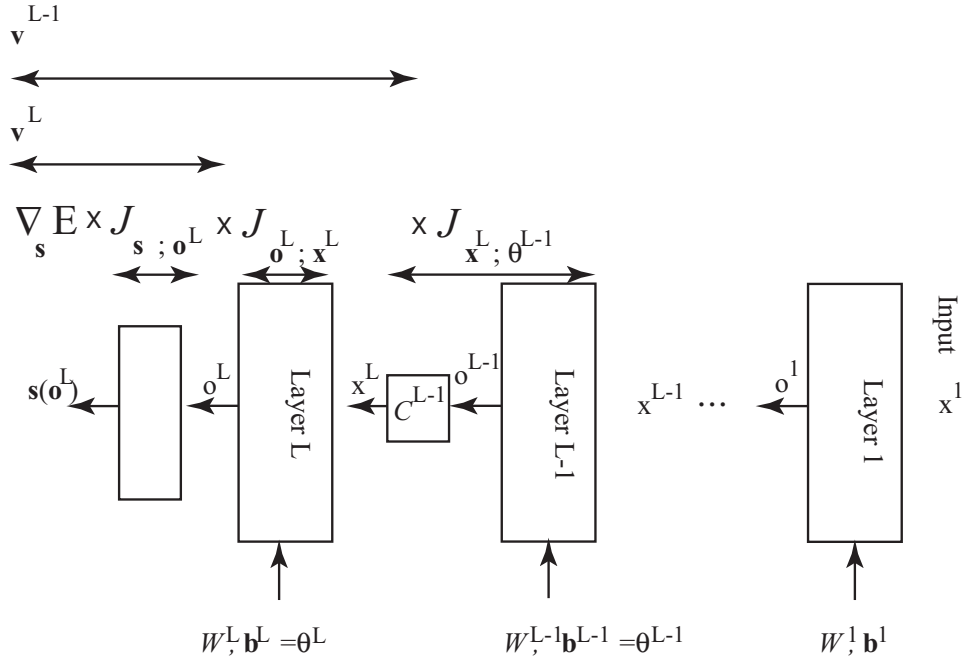
FIGURE 11.5: Constructing the gradient with respect to \theta^{L-1} .
