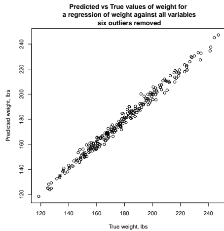
FIGURE 5.18: A scatter plot of the predicted weight against the true weight for the bodyfat dataset. The prediction is made with all variables, but the six outliers identified above are omitted. I used a Box-Cox transformation with parameter 1/2 , and the regularization parameter that yielded the smallest mean square error in Figure 5.17.
