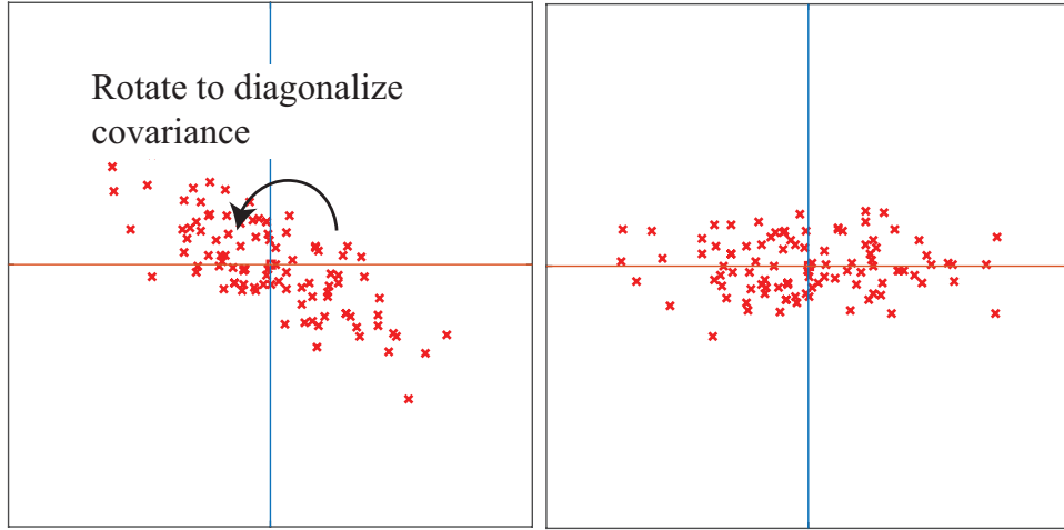
FIGURE 2.6: On the left, the translated blob of figure 2.5. This blob lies somewhat diagonally, because the vertical and horizontal components are correlated. On the right, that blob of data rotated so that there is no correlation between these components. We can now describe the blob by the vertical and horizontal variances alone, as long as we do so in the new coordinate system. In this coordinate system, the vertical variance is significantly larger than the horizontal variance — the blob is short and wide.
