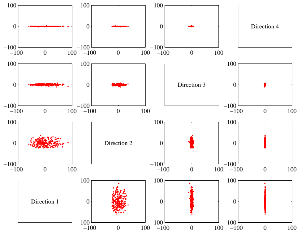
FIGURE 2.8: A panel plot of the bodyfat dataset of figure 2.4, now rotated so that the covariance between all pairs of distinct dimensions is zero. Now we do not know the names for the directions — they’re linear combinations of the original variables. Each scatterplot is on the same set of axes, so you can see that the dataset extends more in some directions than in others.
