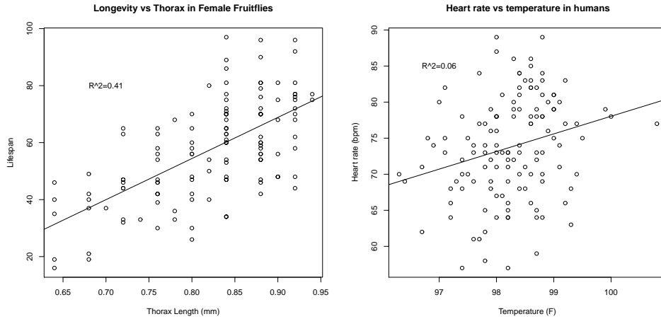
FIGURE 5.2: Regressions do not necessarily yield good predictions or good model fits. On the left, a regression of the lifespan of female fruitflies against the length of their torso as adults (apparently, this doesn't change as a fruitfly ages; you can find this dataset, and the back story at http://www.amstat.org/publications/jse/jse_data_archive.htm ; look for “fruitfly” on that page). The figure suggests you can make some prediction of how long your fruitfly will last by measuring its torso, but not a particularly accurate one. On the right, a regression of heart rate against body temperature for adults. You can find the data at http://www.amstat.org/publications/jse/jse_data_archive.htm as well; look for “temperature” on that page. Notice that predicting heart rate from body temperature isn't going to work that well, either.
