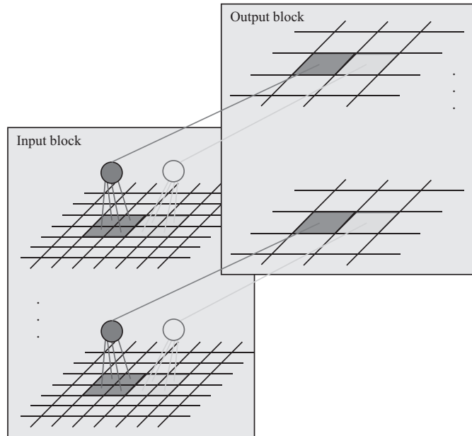
FIGURE 11.12: In a pooling layer, pooling units compute the largest value of their inputs, then pass it on. The most common case is 2 \times 2 , illustrated here. We tile each slice with 2 \times 2 windows that do not overlap. Pooling units compute the max, then pass that on to the corresponding location in the corresponding slice of the output block. As a result, the spatial dimensions of the output block will be about half those of the input block (details depend on how one handles windows that hang over the edge).
