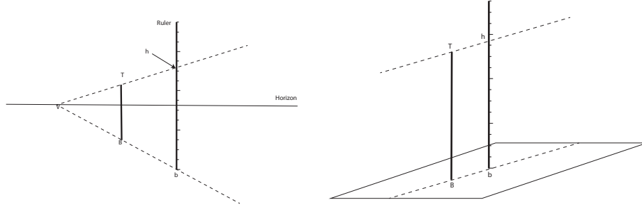
FIGURE 32.3: Left , an image of a ruler and an object, which just happen to be standing perpendicular to a ground plane. In an uncalibrated image like this, we can measure the height of the object. Construct the line bB , and intersect that with the horizon to get the point V . The line from the top of the object T to the true height of the object on the ruler ( h ) is parallel in 3D to bB . In turn, the line Th must intersect the horizon at V . So if you construct VT , it will intersect the ruler at h yielding the height of the object. Right shows a 3D view; the line Th must be parallel to bB , and so in the image these two lines intersect at the horizon.
