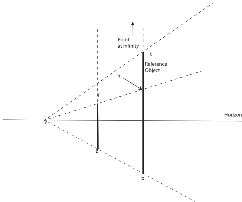
FIGURE 32.6: A perspective camera views a reference object and another object perpendicular to a ground plane. This produces a line segment in the image plane. Constructing appropriate lines in the figure and taking a cross ratio yields the height of the object.
