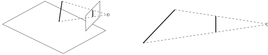
FIGURE 32.5: Left , a perspective camera views a reference object perpendicular to a ground plane. This produces a line segment in the image plane. Right shows the reference object and the line segment in the image plane.
