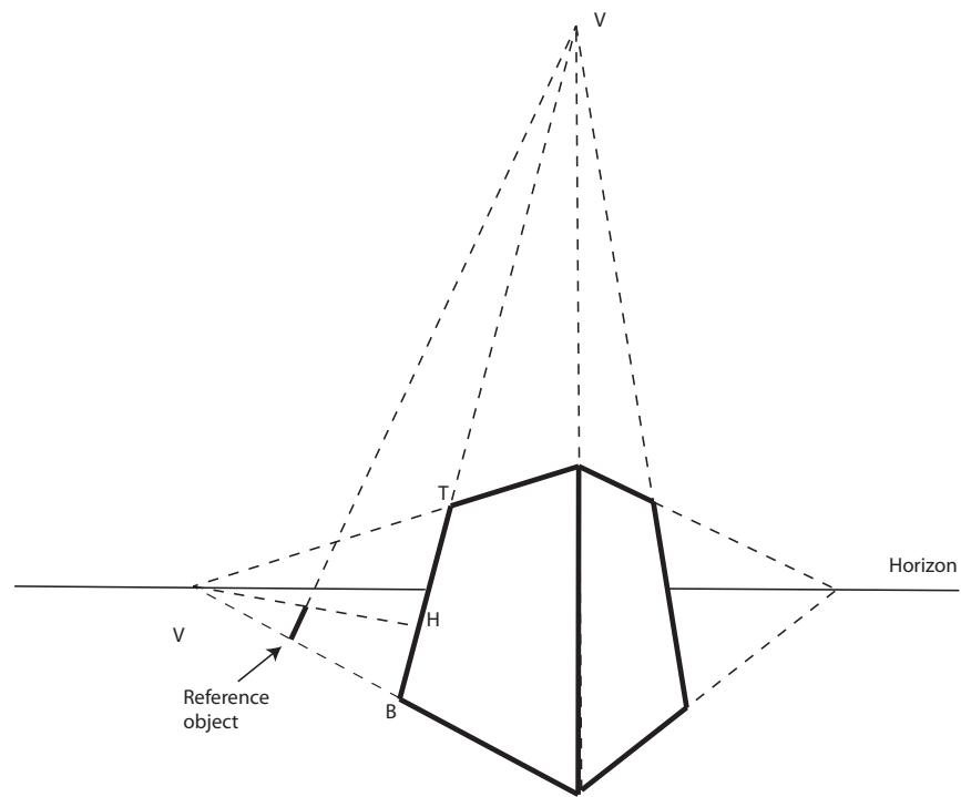
FIGURE 32.7: A building and a person viewed in a more extreme perspective view than that of 32.6. The person has known height, and can act as reference object. The same construction as in that figure yields the height of the building relative to the person.
