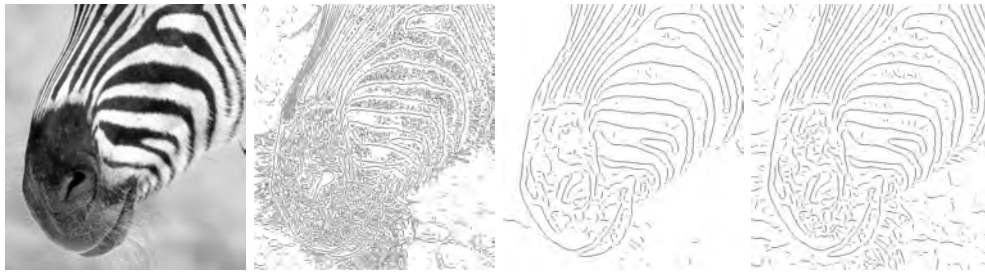
FIGURE 8.4: Edge points marked on the pixel grid for the image shown on the left . The edge points on the center left are obtained using a Gaussian smoothing filter at \sigma one pixel, and gradient magnitude has been tested against a high threshold to determine whether a point is an edge point. The edge points at the center right are obtained using a Gaussian smoothing filter at \sigma four pixels, and gradient magnitude has been tested against a high threshold to determine whether a point is an edge point. The edge points on the right are obtained using a Gaussian smoothing filter at \sigma four pixels, and gradient magnitude has been tested against a low threshold to determine whether a point is an edge point. At a fine scale, fine detail at high contrast generates edge points, which disappear at the coarser scale. When the threshold is high, curves of edge points are often broken because the gradient magnitude dips below the threshold; for the low threshold, a variety of new edge points of dubious significance are introduced.
