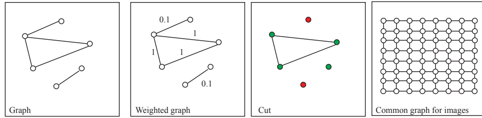
FIGURE 9.7: Graphs are quite visual concepts. On the left , a graph (vertices are circles, and edges line segments; note this graph isn't connected). Center left , a weighted graph; center right , a cut (red vertices are in \mathcal{A} and green vertices are in \mathcal{B} ; and right , the most usual graph used for images, shown for a small image.
