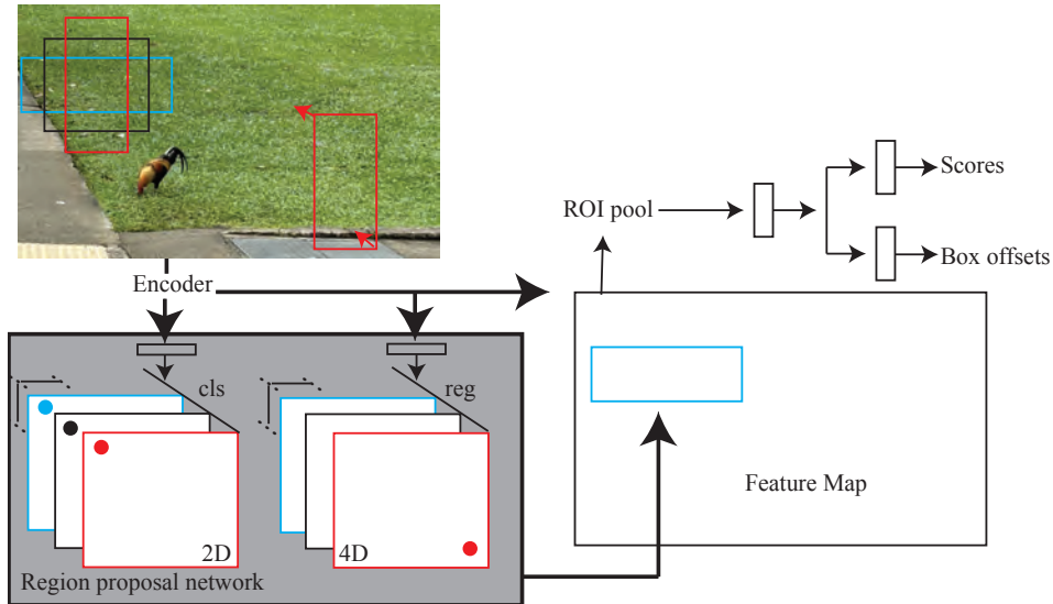
FIGURE 26.1: Faster R-CNN takes a feature description from an encoder, and produces a set of boxes with object category scores for each. Anchor boxes (colored boxes on top left of image) are samples in configuration space. Their N_x \times N_y centers are on an x - y grid, and there are three aspect ratios (shown) and three scales (suppressed). A region proposal network (RPN) produces object/no object scores for each box in a cls block (size N_x \times N_y \times (2 \times 9) , so two scores per box; the color shows how a location in cls corresponds to a box in an image). The RPN produces a reg block consisting of four offset values for each box (size N_x \times N_y \times (4 \times 9) ; the red shows how the offset adjusts the basic anchor box). The boxes are supplied to a ROI pooling layer, which computes a fixed size vector for each box from the piece of the encoded image that corresponds to the underlying box. This vector is passed to a fully connected layer that constructs a large feature, which in turn is fed to two fully connected layers. One produces a score for each category in a box, and the other produces a per category offset for the box.
