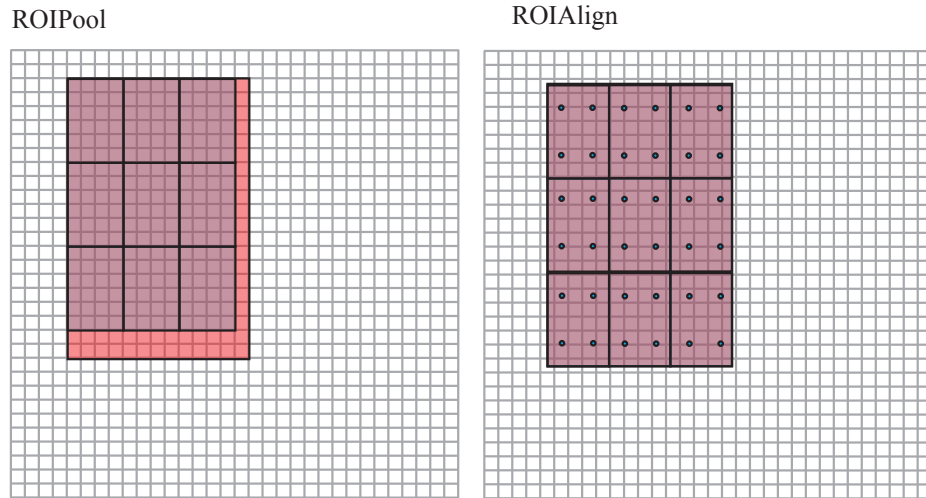
FIGURE 26.2: On the left , ROIPool reduces a feature map to a fixed size feature by max pooling in a set of boxes (the translucent gray boxes). The feature sample is located at the center of each box. The ROI on the feature map (the translucent red box) is determined by rounding as is the placement of the pooling boxes, leading to a loss of spatial information. Notice how some parts of the ROI don't contribute, because of the rounding. On the right , ROIAlign places the ROI exactly on the feature map, samples at a grid of points ( blue ) inside each box using bilinear interpolation, then pools these samples inside each box. This preserves spatial information. Numerical details in the text.
