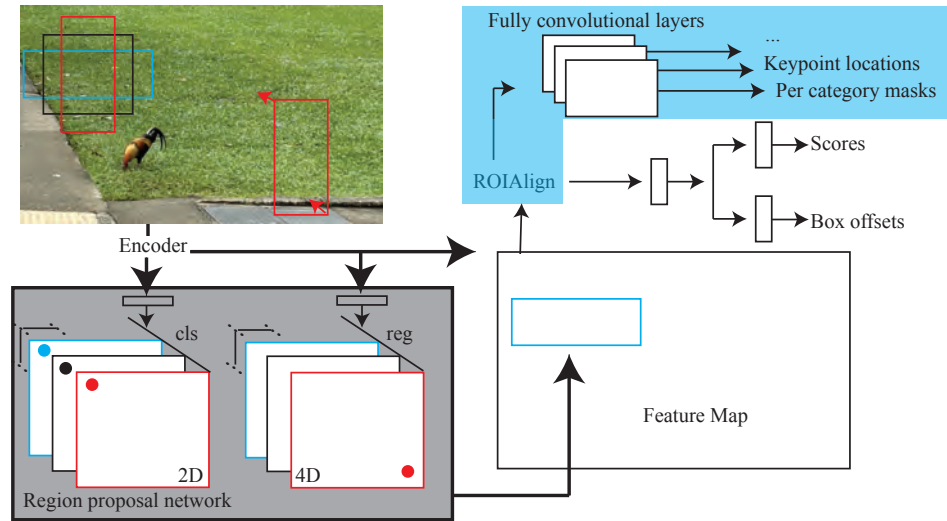
FIGURE 26.4: MaskRCNN involves small but significant modifications to FasterRCNN which are indicated in the blue boxes (compare to Figure 26.1). ROI Pool is replaced with ROIAlign ; and the results are passed through a fully convolutional network to produce a set of fixed size masks, one per category. This procedure can be applied to other predictions as well. I describe keypoint predictions in the text, but the figure leaves room for other possibilities.
