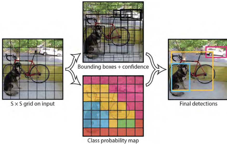
FIGURE 26.5: YOLO predicts a confidence score for a set of B boxes in each of an S \times S grid of tiles together with a class posterior score for each object category at each tile. These scores are combined to produce the score for boxes. The resulting boxes are then post processed (non-maximum suppression) and reported. Image Credit: Figure 2 of You Only Look Once: Unified, Real-Time Object Detection Joseph Redmon, Santosh Divvala, Ross Girshick, Ali Farhadi
