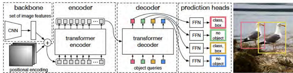
FIGURE 26.9: Image Credit: Part of Figure 1 of End-to-End Object Detection with Transformers Nicolas Carion?, Francisco Massa?, Gabriel Synnaeve, Nicolas Usunier, Alexander Kirillov, and Sergey Zagoruyko
