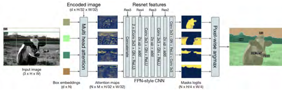
FIGURE 26.10: Image Credit: Part of Figure 8 of End-to-End Object Detection with Transformers Nicolas Carion?, Francisco Massa?, Gabriel Synnaeve, Nicolas Usunier, Alexander Kirillov, and Sergey Zagoruyko
