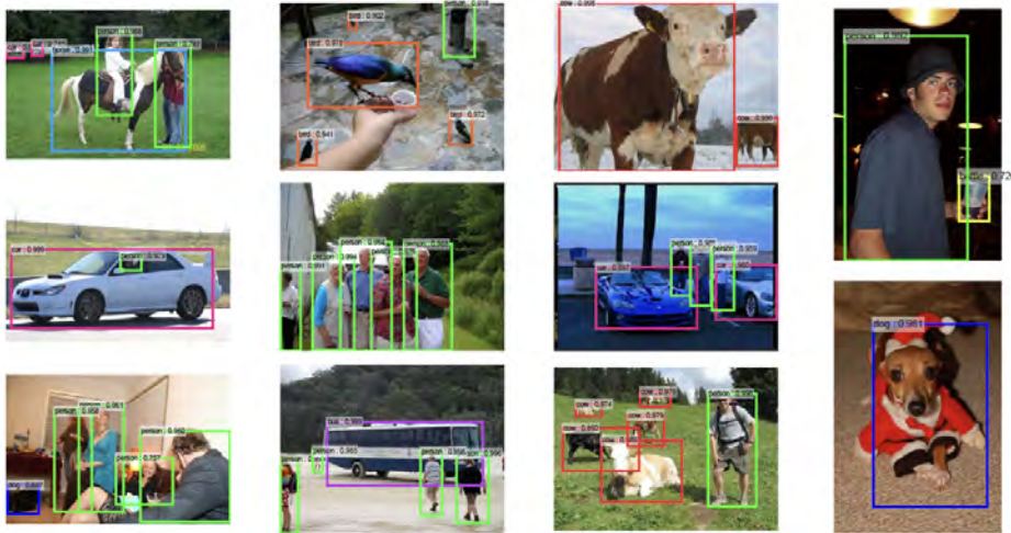
FIGURE 26.3: Detection results using Faster R-CNN on parts of the PASCAL VOC 2007 test set. Image Credit: Figure 2 of Faster R-CNN: Towards Real-Time Object Detection with Region Proposal Networks Shaoqing Ren, Kaiming He, Ross Girshick, and Jian Sun
