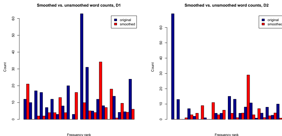
FIGURE 5.5: Unsmoothed and smoothed word counts for two different documents, where smoothing is by LSA to 1000 intermediate dimensions. Each figure shows one document; the blue bars are unsmoothed counts and the red bars are smoothed counts. The figure shows the counts for the 100 words that appear most frequently in the whole dataset, ordered by the rank of the word count (most common word first, etc.) Notice that generally, large counts tend to go down, and small counts tend to go up, as one would expect.
