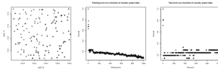
FIGURE 17.5: On the left, a scatter plot of the prawn data. The circles are locations where the prawn catch exceeded the median; the stars are locations where the catch was below median. Center shows the training error for a boosted classifier using decision stumps, as a function of the number of stumps. Notice how adding a stump causes the training error to fall slowly but reliably even when we already have many predictors. Right shows the test error, which settles close to a fixed value fairly quickly. This isn't typical behavior – it is common to observe the test error falling reliably as well. Figure ?? visualizes the predictors.
