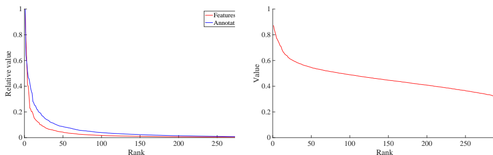
FIGURE 6.1: On the left , the 291 largest eigenvalues of the covariance for features and for word vectors, normalized by the largest eigenvalue in each case, plotted against rank. Notice in each case relatively few eigenvalues capture most of the variance. The word vectors are 291 dimensional, so this figure shows all the variances for the word vectors, but there are a total of 3000 eigenvalues for the features. On the right , the canonical correlations for this data set. Notice that there are some rather large correlations, but quite quickly the values are small.
