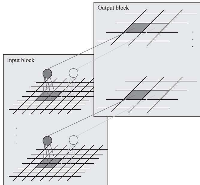
FIGURE 15.11: In a pooling layer, pooling units compute the largest value of their inputs, then pass it on. The most common case is 2 \times 2 , illustrated here. We tile each slice with 2 \times 2 windows that do not overlap. Pooling units compute the max, then pass that on to the corresponding location in the corresponding slice of the output block. As a result, the spatial dimensions of the output block will be about half those of the input block (details depend on how one handles windows that hang over the edge).
