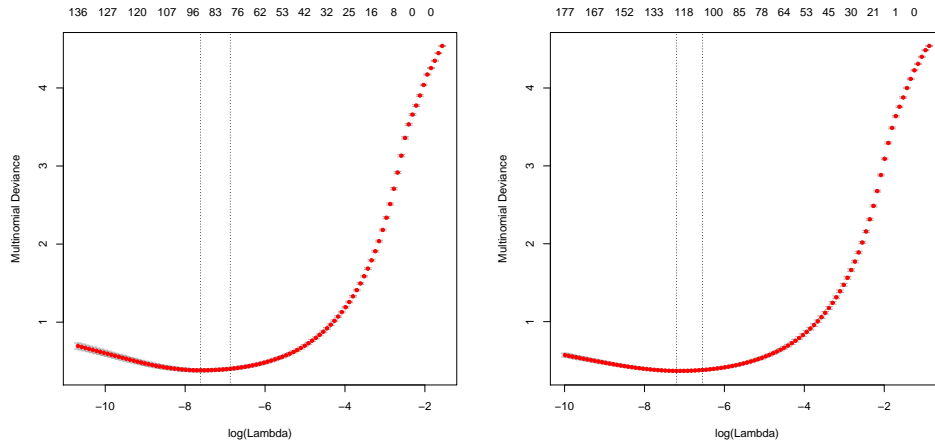
FIGURE 10.9: Multiclass logistic regression on the MNIST data set, using a lasso and elastic net regularizers. On the left , deviance of held out data on the digit data set (worked example 10.6), for different values of the log regularization parameter in the lasso case. On the right , deviance of held out data on the digit data set (worked example 10.6), for different values of the log regularization parameter in the elastic net case, \alpha = 0.5 .
