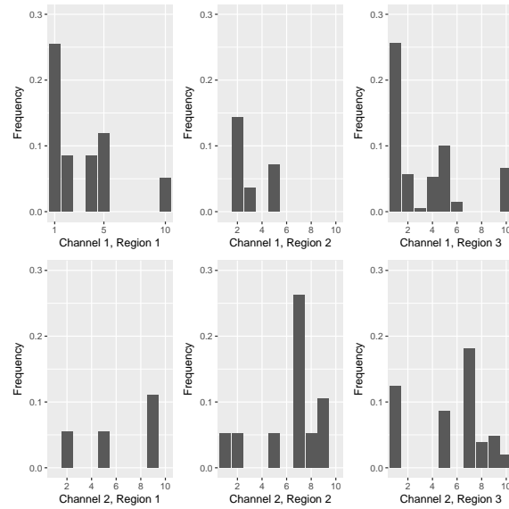
FIGURE 7.11: The histogram of different types of customer, by group, for the customer data. Notice how the distinction between the groups is now apparent — the groups do appear to contain quite different distributions of customer type. It looks as though the channels (rows in this figure) are more different than the regions (columns in this figure).
