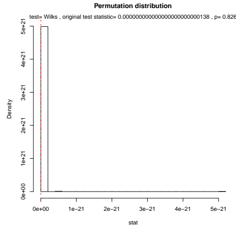
FIGURE 6.9: A histogram of values of Wilks' lambda obtained from permuted versions of the 400 tile albedo shading dataset discussed in the text. The value obtained for the original dataset is shown by the vertical line, and is really tiny (rather less than 1e-21 ). But rather more than four-fifths (82.6%) of the values obtained by permuting the data are even tinier, meaning that we would see the canonical correlation values we see or smaller about 4 in every 5 experiments if they were purely a chance effect. There is no reason to believe the two have a correlation.
