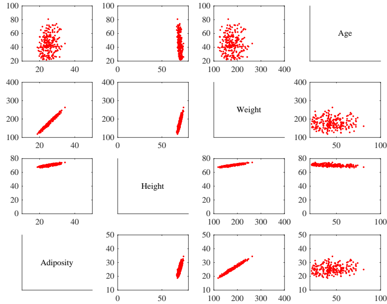
FIGURE 4.4: The data of Figure 3.4, represented by translating and rotating so that the covariance is diagonal, projecting off the two smallest directions, then undoing the rotation and translation. This blob of data is two dimensional (because we projected off two dimensions – figure 4.2 suggested this was safe), but is represented in a four dimensional space. You can think of it as a thin two dimensional pancake of data in the four dimensional space (you should compare to Figure 3.4 on page 64). It is a good representation of the original data. Notice that it looks slightly thickened on edge, because it isn't aligned with the coordinate system – think of a view of a flat plate at a slight slant.
