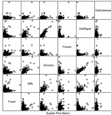
FIGURE 7.9: A panel plot of the wholesale customer data of http://archive.ics.uci.edu/ml/datasets/Wholesale+customers , which records sums of money spent annually on different commodities by customers in Portugal. This data is recorded for six different groups (two channels each within three regions). I have plotted each group with a different marker, but you can't really see much structure here, for reasons explained in the text.
