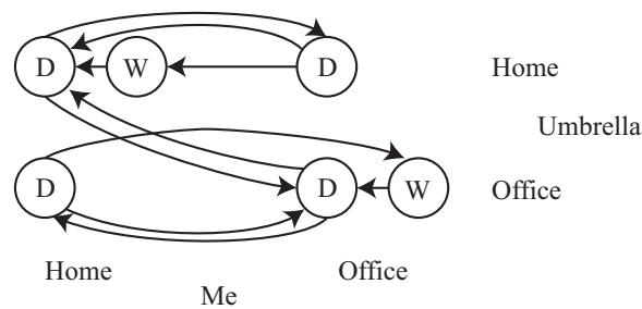
FIGURE 11.1: A directed graph representing the umbrella example. Notice you can't arrive at the office wet with the umbrella at home (you'd have taken it), and so on. Labelling the edges with probabilities is left to the reader.
