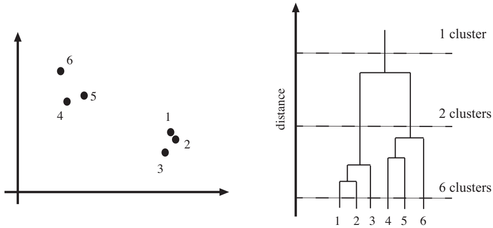
FIGURE 7.1: Left , a data set; right , a dendrogram obtained by agglomerative clustering using single-link clustering. If one selects a particular value of distance, then a horizontal line at that distance splits the dendrogram into clusters. This representation makes it possible to guess how many clusters there are and to get some insight into how good the clusters are.
