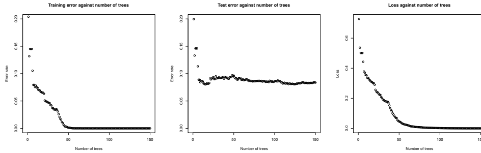
FIGURE 17.7: Models for a boosted decision tree classifier predicting whether a given prescriber will write more than 10 opioid prescriptions in a year, using the data of https://www.kaggle.com/apryor6/us-opiate-prescriptions . Left: training error against number of trees; center: test error against number of trees; right: exponential loss against number of trees. Notice that both test and train error go down, but there is a test-train gap. Notice also a characteristic property of boosting; continuing to boost after the training error is zero (about 50 trees in this case) still results in improvements in the test error. Note also that lower exponential loss doesn't guarantee lower training error.
