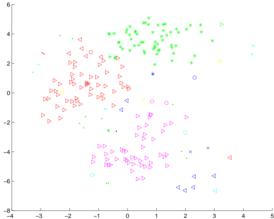
FIGURE 7.3: A clustering of the seed dataset, using agglomerative clustering, single link distance, and requiring a maximum of 30 clusters. I have plotted each cluster with a distinct marker (though some markers differ only by color). Notice that there are a set of fairly natural isolated clusters. The original data is 8 dimensional, which presents plotting problems; I show a scatter plot on the first two principal components (though I computed distances for clustering in the original 8 dimensional space).
