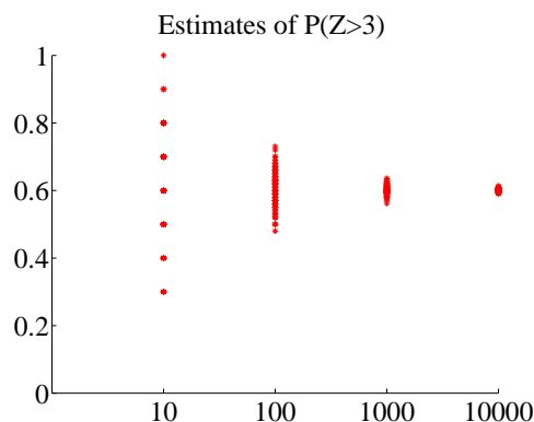
FIGURE 11.6: Estimates of the probability from example 11.11, obtained from different runs of my simulator using different numbers of samples. In each case, I used 100 runs; the number of samples is shown on the horizontal axis. You should notice that the estimate varies pretty widely when there are only 10 samples in each run, but the variance (equivalently, the size of the spread) goes down sharply as the number of samples per run increases to 1000. Because we expect these estimates to be roughly normally distributed, the variance gives a good idea of how accurate the original probability estimate is.
