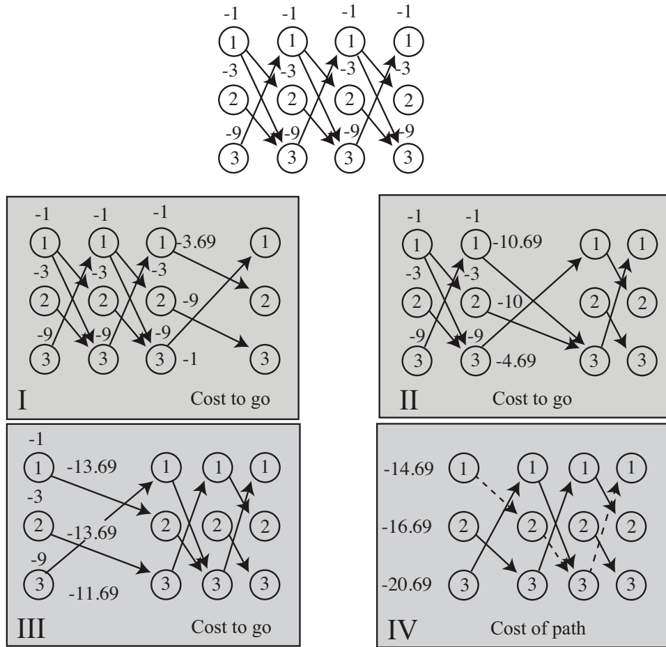
FIGURE 12.2: An example of finding the best path through a trellis. The probabilities of leaving a node are uniform (and remember, \ln 2 \approx -0.69 ). Details in the text.
