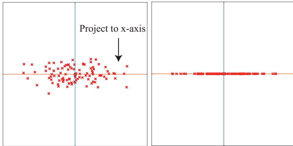
FIGURE 4.1: On the left , the translated and rotated blob of figure 3.6. This blob is stretched — one direction has more variance than another. Setting the y coordinate to zero for each of these datapoints results in a representation that has relatively low error, because there isn't much variance in these values. This results in the blob on the right . The text shows how the error that results from this projection is computed.
