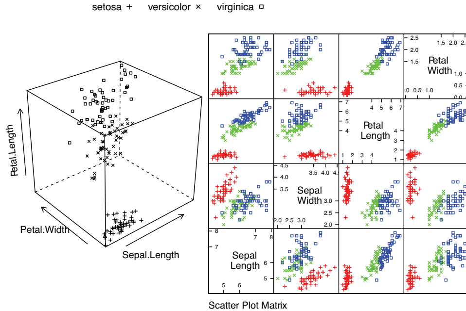
FIGURE 7.4: Left: a 3D scatterplot for the famous Iris data, collected by Edgar Anderson in 1936, and made popular amongst statisticians by Ronald Fisher in that year. I have chosen three variables from the four, and have plotted each species with a different marker. You can see from the plot that the species cluster quite tightly, and are different from one another. Right: a scatterplot matrix for the Iris data. There are four variables, measured for each of three species of iris. I have plotted each species with a different marker. You can see from the plot that the species cluster quite tightly, and are different from one another.
