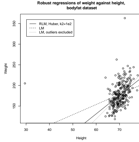
FIGURE 10.2: Comparing three different linear regression strategies on the bodyfat data, regressing weight against height. Notice that using an M -estimator gives an answer very like that obtained by rejecting outliers by hand. The answer may well be “better” because it isn’t certain that each of the four points rejected is an outlier, and the robust method may benefit from some of the information in these points. I tried a range of scales for the Huber loss (the ‘ k2 ’ parameter), but found no difference in the line resulting over scales varying by a factor of 1e4 , which is why I plot only one scale.
