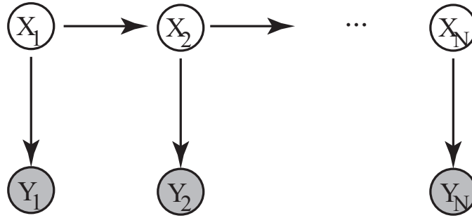
FIGURE 13.1: An HMM is an example of a graphical model. The joint probability distribution of the hidden variables X_i and the observations Y_i factors as in the text. Each variable appears as a vertex. There is an edge between pairs of variables that appear in the factorization. These edges have an arrowhead drawn according to conventions about conditional probability. Finally, the observed values are shaded.
