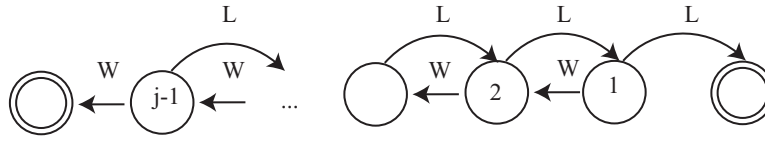
FIGURE 11.2: A directed graph representing the gambler's ruin example. I have labelled each state with the amount of money the gambler has at that state. There are two end states, where the gambler has zero (is ruined), or has j and decides to leave the table. The problem we discuss is to compute the probability of being ruined, given the start state is s . This means that any state except the end states could be a start state. I have labelled the state transitions with "W" (for win) and "L" for lose, but have omitted the probabilities.
