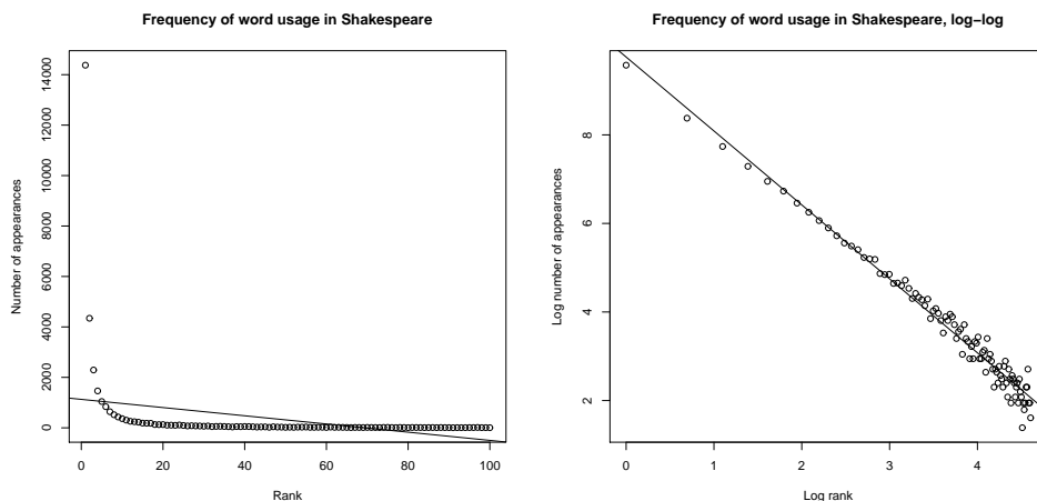
FIGURE 9.4: On the left , word count plotted against rank for the 100 most common words in Shakespeare, using a dataset that comes with R (called “bard”, and quite likely originating in an unpublished report by J. Gani and I. Saunders). I show a regression line too. This is a poor fit by eye, and the R^2 is poor, too ( R^2 = 0.1 ). On the right , log word count plotted against log rank for the 100 most common words in Shakespeare, using a dataset that comes with R (called “bard”, and quite likely originating in an unpublished report by J. Gani and I. Saunders). The regression line is very close to the data.
