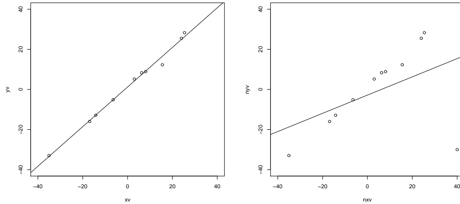
FIGURE 9.6: On the left, a synthetic dataset with one independent and one explanatory variable, with the regression line plotted. Notice the line is close to the data points, and its predictions seem likely to be reliable. On the right, the result of adding a single outlying datapoint to that dataset. The regression line has changed significantly, because the regression line tries to minimize the sum of squared vertical distances between the data points and the line. Because the outlying datapoint is far from the line, the squared vertical distance to this point is enormous. The line has moved to reduce this distance, at the cost of making the other points further from the line.
