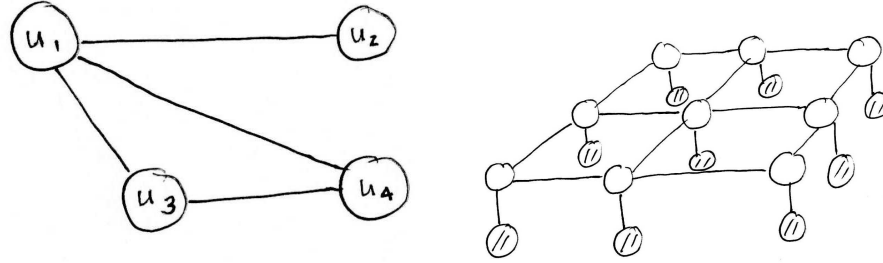
FIGURE 14.1: On the left , a simple Boltzmann machine. Each U_i has two possible states, so the whole thing has 16 states. Different choices of the constants coupling the U 's along each edge lead to different probability distributions. On the right , this Boltzmann machine adapted to denoising binary images. The shaded nodes represent the known pixel values ( X_i in the text) and the open nodes represent the (unknown, and to be inferred) true pixel values H_i . Notice that pixels depend on their neighbors in the grid.
