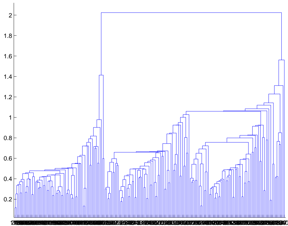
FIGURE 7.2: A dendrogram obtained from the seed dataset, using single link clustering. Recall that the data points are on the horizontal axis, and that the vertical axis is distance; there is a horizontal line linking two clusters that get merged, established at the height at which they're merged. I have plotted the entire dendrogram, despite the fact it's a bit crowded at the bottom, because you can now see how clearly the data set clusters into a small set of clusters — there are a small number of vertical “runs”.
