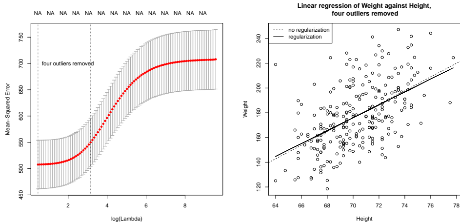
FIGURE 9.12: On the left , cross-validated error estimated for different choices of regularization constant for a linear regression of weight against height for the bodyfat dataset, with four outliers removed. The horizontal axis is log regression constant; the vertical is cross-validated error. The mean of the error is shown as a spot, with vertical error bars. The vertical lines show a range of reasonable choices of regularization constant ( left yields the lowest observed error, right the error whose mean is within one standard error of the minimum). On the right , two regression lines on a scatter plot of this dataset; one is the line computed without regularization, the other is obtained using the regularization parameter that yields the lowest observed error. In this case, the regularizer doesn't change the line much, but may produce improved values on new data (notice how the cross-validated error is fairly flat with low values of the regularization constant).
