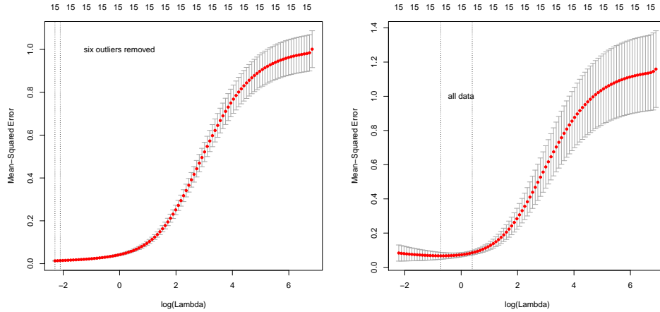
FIGURE 9.17: Plots of mean-squared error as a function of log regularization parameter (i.e. \log \lambda ) for a regression of \text{weight}^{1/2} against all variables for the bodyfat dataset. These plots show mean-squared error averaged over cross-validation folds with a vertical one standard deviation bar. On the left , the plot for the dataset with the six outliers identified in Figure 287 removed. On the right , the plot for the whole dataset. Notice how the outliers increase the variability of the error, and the best error.
