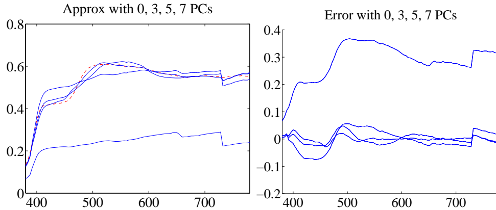
FIGURE 4.6: On the left , a spectral reflectance curve (dashed) and approximations using the mean, the mean and 3 principal components, the mean and 5 principal components, and the mean and 7 principal components. Notice the mean is a relatively poor approximation, but as the number of principal components goes up, the mean squared distance between measurements and principal component representation falls rather quickly. On the right is this distance for these approximations. A projection onto very few principal components suppresses local wiggles in the data unless very many data items have the same wiggle in the same place. As the number of principal components increases, the representation follows the measurements more closely. The best estimate of each component of a data item is likely not the measurement – it’s a prediction obtained from all measurements. The projection onto principal components is such a prediction, and you can see the smoothing effects of principal components analysis in these plots. Figure plotted from a dataset of 1995 spectral reflectances, collected by Kobus Barnard (at http://www.cs.sfu.ca/~colour/data/ ).
