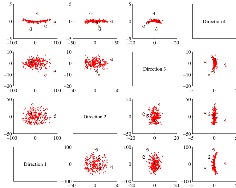
FIGURE 4.3: A panel plot of the bodyfat dataset of figure 3.4, now rotated so that the covariance between all pairs of distinct dimensions is zero. Now we do not know names for the directions — they’re linear combinations of the original variables. Compare this figure with figure 4.3; in that figure, the axes were the same, but in this figure I have scaled the axes so you can see details. Notice that the blob is a little curved, and there are several data points that seem to lie some way away from the blob, which I have numbered.
