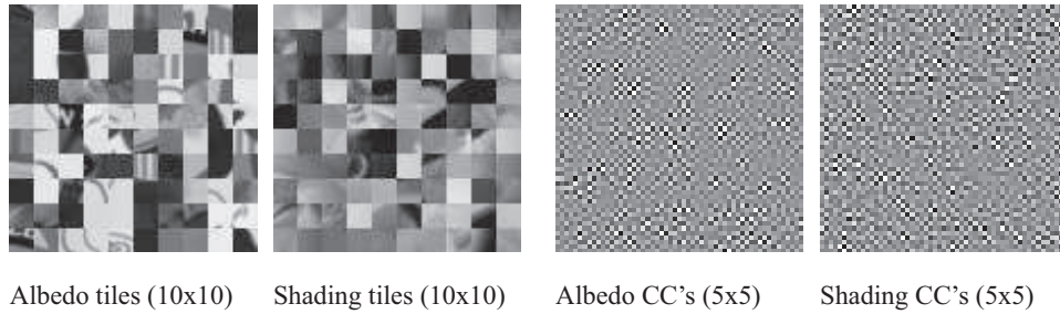
FIGURE 6.6: On the left, a 10 \times 10 grid of tiles of albedo (far left) and shading (center left), taken from Grosse et al's data set. The position of the tiles is keyed, so (for example) the albedo tile at 3, 5 corresponds to the shading tile at 3, 5. On the right, the first 25 canonical correlation directions for albedo (center right) and shading (far right). I have reshaped these into tiles and zoomed them. The scale is smallest value is black, and largest white. These are ordered so the pair with highest correlation is at the top left, next highest is one step to the right, etc. You should notice that these directions do not look even slightly like the patterns in the original tiles, or like any pattern you expect to encounter in a real image. This is because they're not: these are directions that have very small variance.
