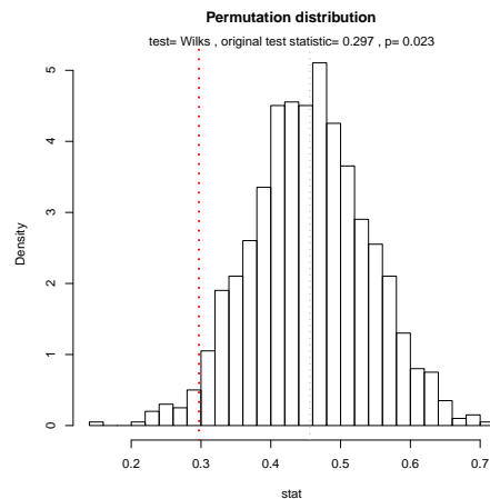
FIGURE 6.7: A histogram of values of Wilks' lambda obtained from permuted versions of the mouse dataset of example 6.1. The value obtained for the original dataset is shown by the vertical line. Notice that most values are larger (about 97% of values), meaning that we would see the canonical correlation values we see only about once in 30 experiments if they were purely a chance effect. There is very likely a real effect here.
