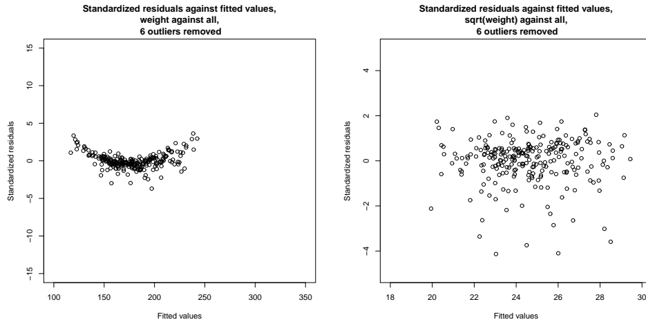
FIGURE 9.16: On the left , standardized residuals plotted against predicted value for weight regressed against all variables for the bodyfat dataset. I removed the four suspicious data points of Figure 9.15, and the two others identified in that figure. Notice a suspicious “banana” shape – the residuals are distinctly larger for small and for large predicted values. This suggests a non-linear transformation of something might be helpful. I used a Box-Cox transformation, which suggested a value of 0.5 (i.e. regress 2(\sqrt{\text{weight}} - 1) ) against all variables. On the right , the standardized residuals for this regression. Notice that the “banana” has gone, though there is a suspicious tendency for the residuals to be smaller rather than larger. Notice also the plots are on different axes. It’s fair to compare these plots by eye; but it’s not fair to compare details, because the residual of a predicted square root means something different than the residual of a predicted value.
