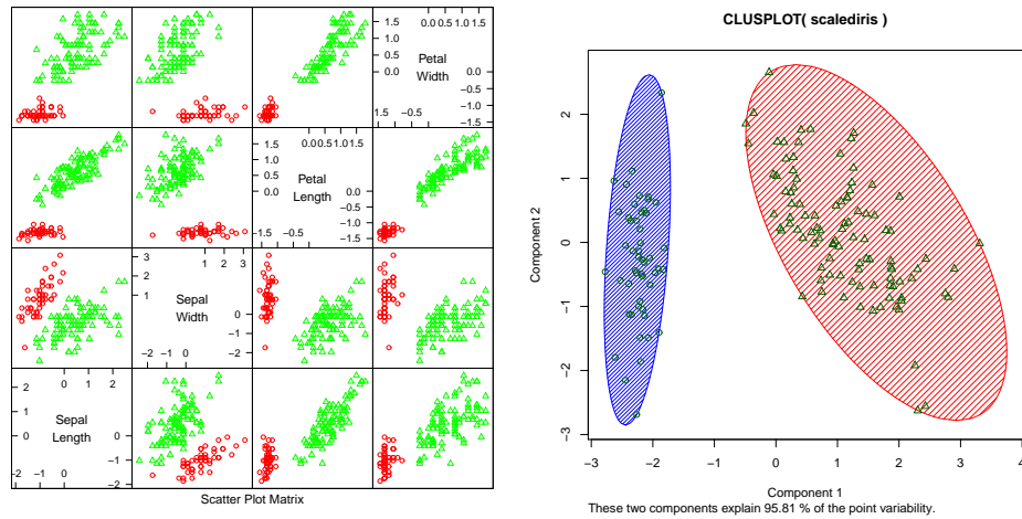
FIGURE 7.5: On the left , a panel plot of the iris data clustered using k -means with k = 2 . By comparison with figure 7.8, notice how the versicolor and virginica clusters appear to have been merged. On the right , this data set projected onto the first two principal components, with one blob drawn over each cluster.
