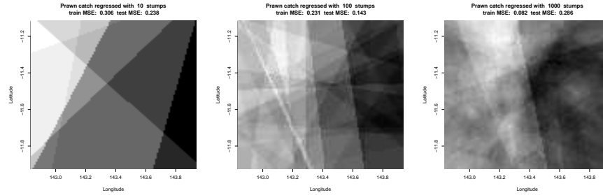
FIGURE 17.6: Visualizations of the predictor for the prawn data of worked example 17.4. Mid-grey is zero; white is positive (and so any shade in the range mid-grey to white predicts a score greater than the median); black is negative (and so any shade in the range mid-grey to black predicts a score less than the median). The predictor formed by one stump cuts the region into two halves with a line; on one side of the line, it takes one constant value, and on the other, it takes a different constant value. Adding many of these together results in a function that is constant in each cell of an arrangement of lines. Predictors that use more stumps produce more complicated functions of this form, with improvements in training error and some improvement in test error (Figure 17.6).
