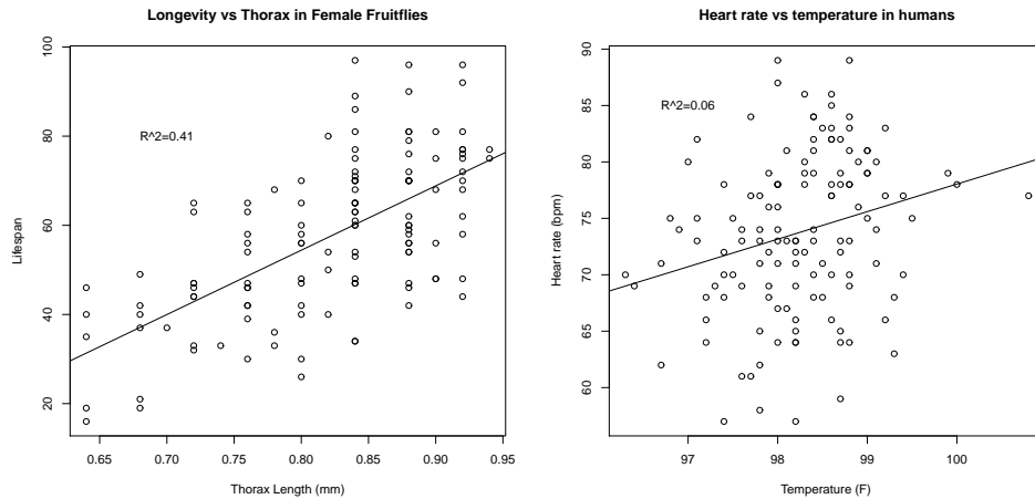
FIGURE 9.2: Regressions do not necessarily yield good predictions or good model fits. On the left, a regression of the lifespan of female fruitflies against the length of their torso as adults (apparently, this doesn't change as a fruitfly ages; you can find this dataset, and the back story at http://www.amstat.org/publications/jse/jse_data_archive.htm ; look for “fruitfly” on that page). The figure suggests you can make some prediction of how long your fruitfly will last by measuring its torso, but not a particularly accurate one. On the right, a regression of heart rate against body temperature for adults. You can find the data at http://www.amstat.org/publications/jse/jse_data_archive.htm as well; look for “temperature” on that page. Notice that predicting heart rate from body temperature isn't going to work that well, either.
