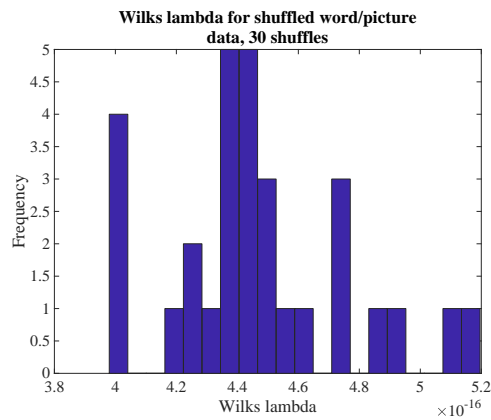
FIGURE 6.8: A histogram of values of Wilks’ lambda obtained from permuted versions of the word and picture dataset of section 6.2. I computed the value for the first 150 canonical variates, and used 30 shuffles (which takes quite a long time). The value for the true dataset is 9.92e - 25 , which suggests very strongly that the correlations are not accidental.
