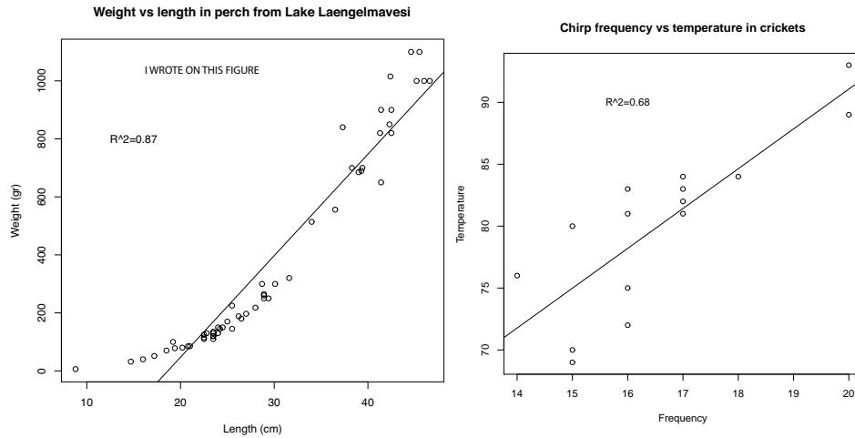
FIGURE 9.1: On the left , a regression of weight against length for perch from a Finnish lake (you can find this dataset, and the back story at http://www.amstat.org/publications/jse/jse_data_archive.htm ; look for “fishcatch” on that page). Notice that the linear regression fits the data fairly well, meaning that you should be able to predict the weight of a perch from its length fairly well. On the right , a regression of air temperature against chirp frequency for crickets. The data is fairly close to the line, meaning that you should be able to tell the temperature from the pitch of cricket’s chirp fairly well. This data is from http://mste.illinois.edu/patel/amar430/keyprob1.html . The R^2 you see on each figure is a measure of the goodness of fit of the regression (section 9.2.4).
