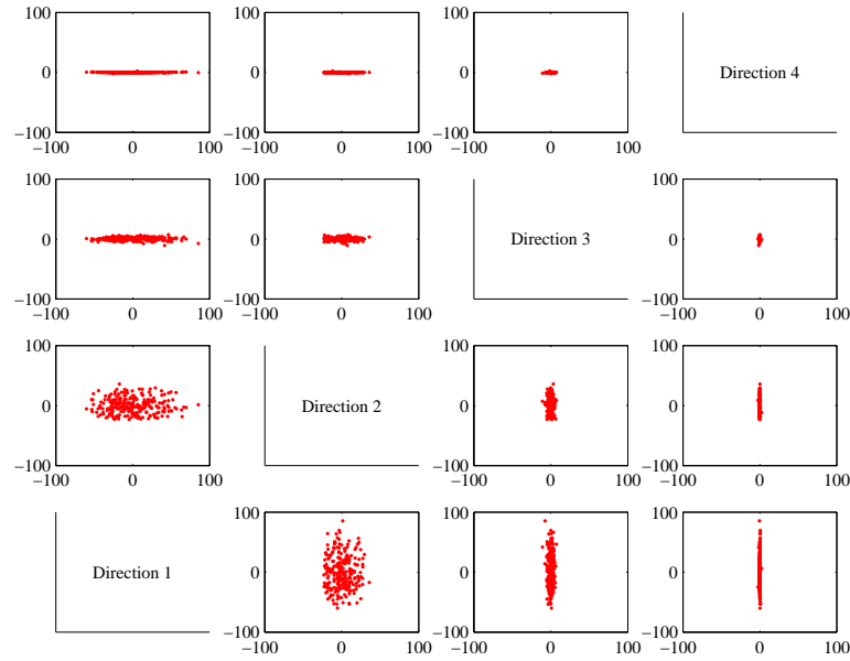
FIGURE 4.2: A panel plot of the bodyfat dataset of figure 3.4, now rotated so that the covariance between all pairs of distinct dimensions is zero. Now we do not know names for the directions — they’re linear combinations of the original variables. Each scatterplot is on the same set of axes, so you can see that the dataset extends more in some directions than in others. You should notice that, in some directions, there is very little variance. This suggests that replacing the coefficient in those directions with zero (as in figure 4.1) should result in a representation of the data that has very little error.
