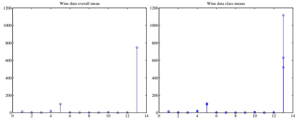
FIGURE 3.2: On the left , a stem plot of the mean of all data items in the wine dataset, from http://archive.ics.uci.edu/ml/datasets/Wine . On the right , I have overlaid stem plots of each class mean from the wine dataset, from http://archive.ics.uci.edu/ml/datasets/Wine , so that you can see the differences between class means.
