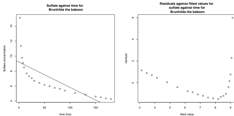
FIGURE 9.22: Left: A regression of the concentration of sulfate in the blood of Brunhilda the baboon against time. Right: For this regression, a plot of residual against fitted value.
