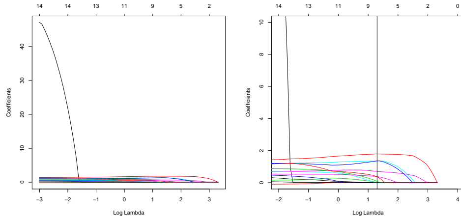
FIGURE 10.5: Plots of coefficient values as a function of \log \lambda for a regression of weight against all variables for the bodyfat dataset, penalised using the L_1 norm. In each case, the six outliers identified in Figure 287 were removed. On the left , the plot of the whole path for each coefficient (each curve is one coefficient). On the right , a detailed version of the plot. The vertical line shows the value of \log \lambda the produces the model with smallest cross-validated error (look at Figure 10.4). Notice that the variable that appears to be important, because it would have a large weight with \lambda = 0 , does not appear in this model.
