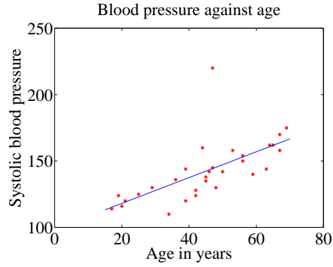
FIGURE 9.19: A regression of blood pressure against age, for 30 data points.
