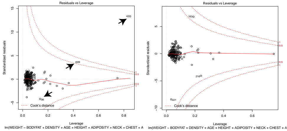
FIGURE 9.14: On the left , residuals plotted against leverage for a regression of weight against all other measurements for the bodyfat dataset. I did not remove the outliers. The contours on the plot are contours of Cook's distance; I have overlaid arrows showing points with suspiciously large Cook's distance. Notice also that several points have high leverage, without having a large residual value. These points may or may not present problems. On the right , the same plot for this dataset with points 36, 39, 41 and 42 removed (these are the points I have been removing for each such plot). Notice that another point now has high Cook's distance, but mostly the residual is much smaller.
