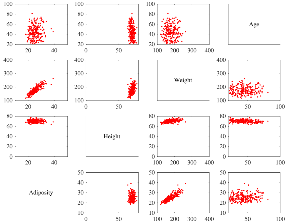
FIGURE 3.4: This is a scatterplot matrix for four of the variables in the height weight dataset of http://www2.stetson.edu/~jrasp/data.htm . Each plot is a scatterplot of a pair of variables. The name of the variable for the horizontal axis is obtained by running your eye down the column; for the vertical axis, along the row. Although this plot is redundant (half of the plots are just flipped versions of the other half), that redundancy makes it easier to follow points by eye. You can look at a column, move down to a row, move across to a column, etc. Notice how you can spot correlations between variables and outliers (the arrows).
