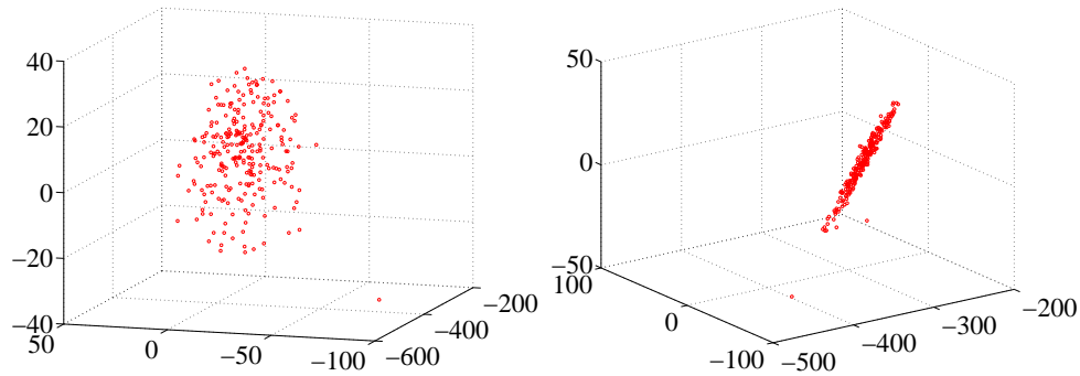
FIGURE 5.3: Two views of a multidimensional scaling to three dimensions of the height-weight dataset. Notice how the data seems to lie in a flat structure in 3D, with one outlying data point. This means that the distances between data points can be (largely) explained by a 2D representation.
