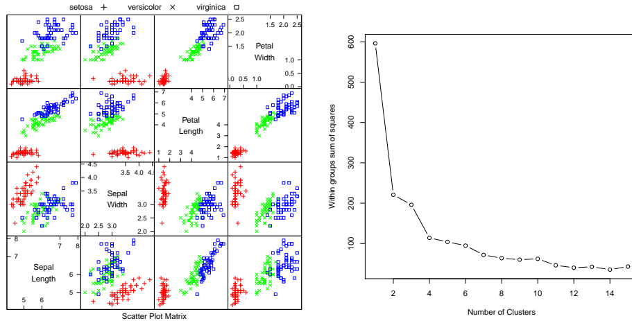
FIGURE 7.8: On the left, the scatterplot matrix for the Iris data, for reference. On the right, a plot of the value of the cost function for each of several different values of k . Notice how there is a sharp drop in cost going from k = 1 to k = 2 , and again at k = 4 ; after that, the cost falls off slowly. This suggests using k = 2 , k = 3 , or k = 4 , depending on the precise application.
