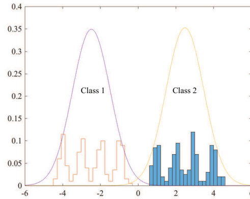
FIGURE 1.1: The figure shows class conditional histograms of a feature x for two different classes. The histograms have been normalized so that the counts sum to one, so you can think of them as probability distributions. It should be fairly obvious that a normal model (superimposed) doesn't describe these histograms well. However, the normal model will result in a good naive bayes classifier.
