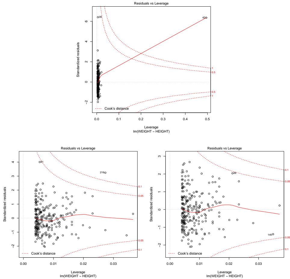
FIGURE 9.10: A diagnostic plot, produced by R, of a linear regression of weight against height for the bodyfat dataset. Top: the whole dataset; bottom left: with the two most extreme points in the top figure removed; bottom right: with two further points (highest residual) removed. Details in text.
