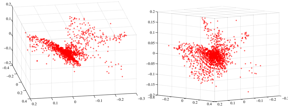
FIGURE 5.2: Two views of the spectral data of section 4.2, plotted as a scatter plot by applying principal coordinate analysis to obtain a 3D set of points. Notice that the data spreads out in 3D, but seems to lie on some structure; it certainly isn't a single blob. This suggests that further investigation would be fruitful.
