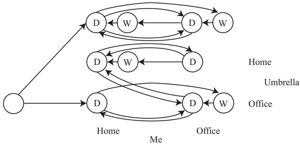
FIGURE 11.5: In this umbrella example, there can't be a stationary distribution; what happens depends on the initial, random choice of buying/not buying an umbrella.
