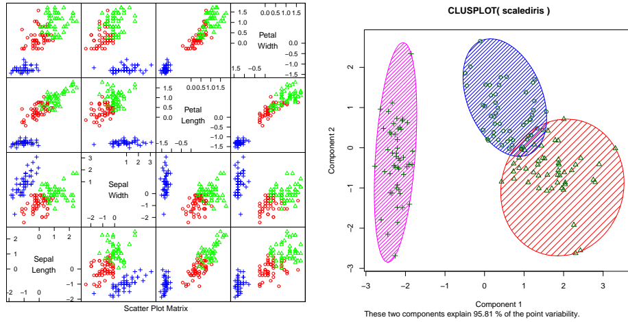
FIGURE 7.6: On the left , a panel plot of the iris data clustered using k -means with k = 3 . By comparison with figure 7.8, notice how the clusters appear to follow the species labels. On the right , this data set projected onto the first two principal components, with one blob drawn over each cluster.
