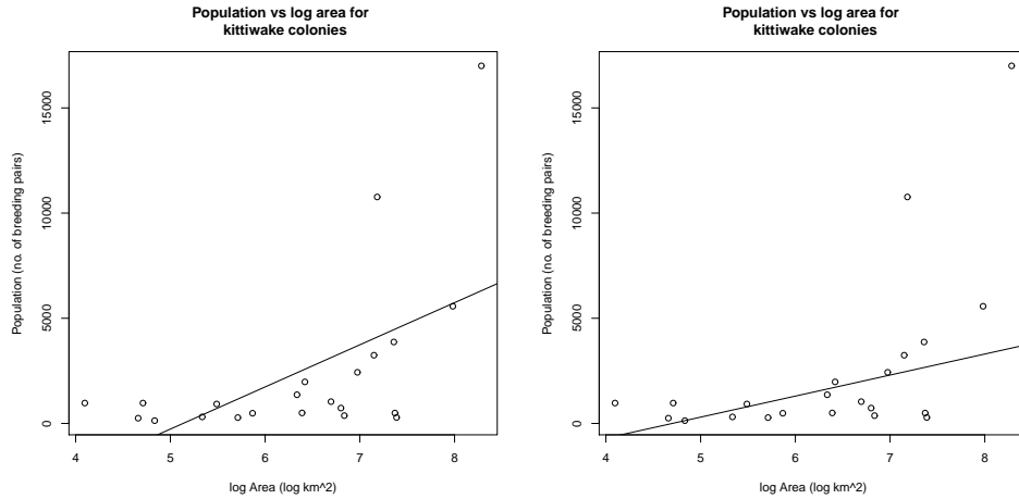
FIGURE 9.21: Left: A regression of the number of breeding pairs of kittiwakes against the log of area of an island, for 22 data points. Right: A regression of the number of breeding pairs of kittiwakes against the log of area of an island, for 22 data points, using a method that ignores two likely outliers.
