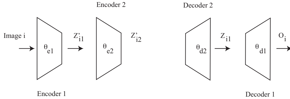
FIGURE 16.3: Two layers of denoising auto-encoder, ready for fine tuning. This figure should help with the notation in the text.
