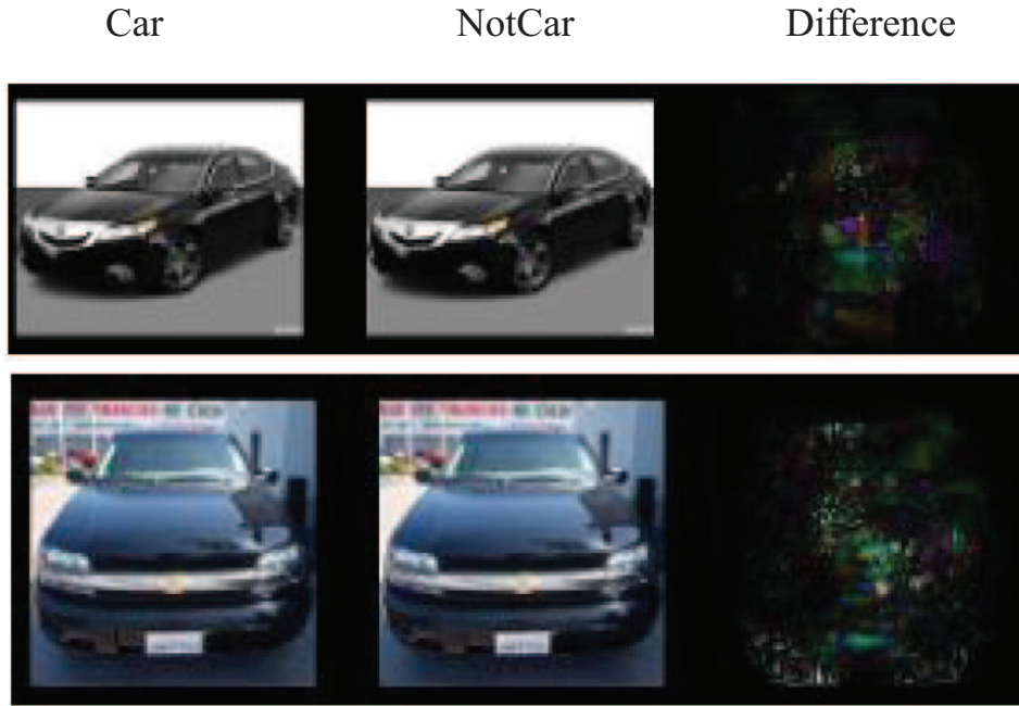
FIGURE 15.15: This figure is from “Intriguing properties of neural networks”, by Christian Szegedy et al.. The left column shows images classified as car ; the middle column shows modified versions of those images classified as not car ; and the right column shows the difference.
