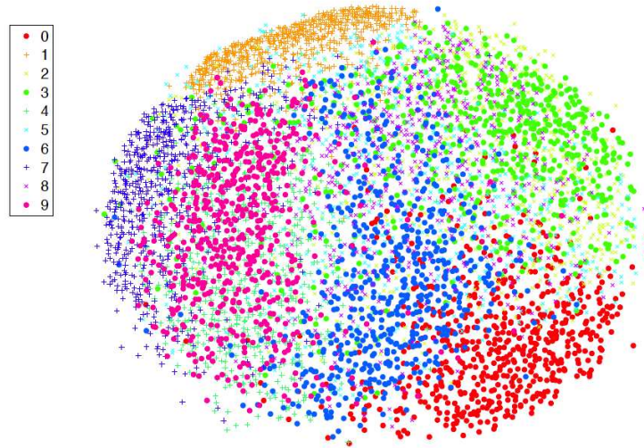
FIGURE 16.1: A Sammon mapping of 6,000 samples of a 1,024 dimensional data set. The data was reduced to 30 dimensions using PCA, then subjected to a Sammon mapping. This data is a set of 6,000 samples from the MNIST dataset, consisting of a collection of handwritten digits which are divided into 10 classes (0,...9). The class labels were not used in training, but the plot shows class labels. This helps determine whether the visualization is any good – you could reasonably expect a visualization to put items in the same class close together and items in very different classes far apart. As the legend on the side shows, the classes are quite well separated. Figure from Visualizing Data using t-SNE Journal of Machine Learning Research 9 (2008) 2579-2605 Laurens van der Maaten and Geoffrey Hinton, to be replaced with a homemade figure in time.
