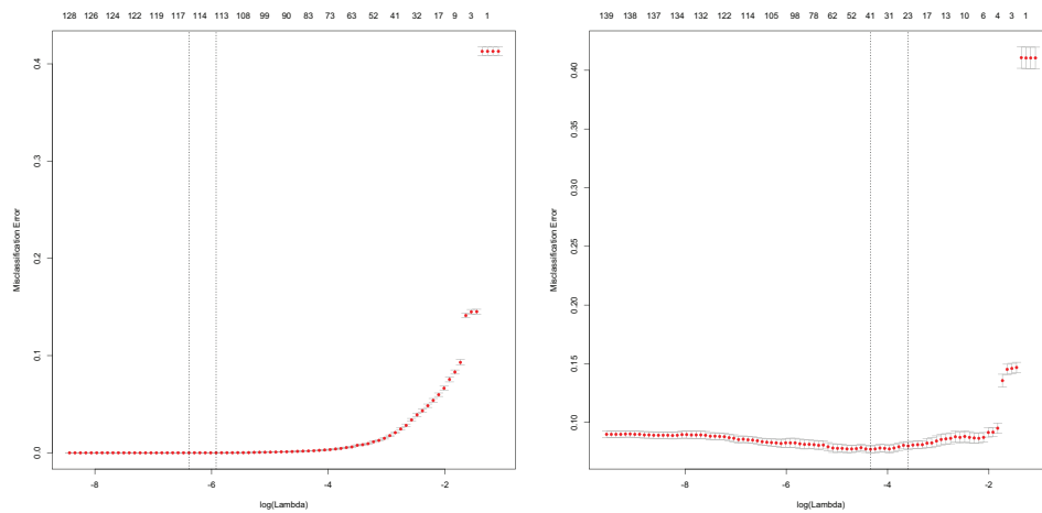
FIGURE 17.8: Left: a cross-validation plot from cv.glmnet for the lasso applied to predictions on training data obtained from all 150 trees from the boosting of figure 17.7. A model with about 113 trees obtains zero error here. Recall from figure 17.7 that training error can be zero; it is here. But this estimate is biased because the trees have been chosen to fit the training data. Right: a cross-validation plot from cv.glmnet using the lasso to choose predictors on data not used to choose the predictors (ie test data). Notice how quite a small model (about 30 trees) achieves the minimum error. This cross-validated estimate of error is not biased, because the trees weren't chosen to fit the data. Notice that this implies a lasso fitted to test must have significantly higher error (it would use about 100 predictors, and you can see what the best such model on training data would do in this curve).
