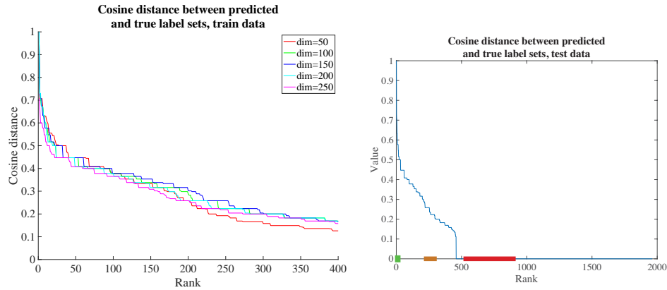
FIGURE 6.5: Left: all values of cosine distance between predicted and true word labels, sorted from best to worst, for the CCA method of the text, for different numbers of canonical variables, for the training data. The distances are fairly good, and 150 seems like a reasonable choice of dimension. On the right , cosine distances between predicted and true for test data; this looks much worse. I have marked the regions where the “good”, “medium” and “bad” figures come from. Note that most values are bad – predicting words from images is hard. Accurate predictions require considerably more sophisticated feature constructions than we have used here.
