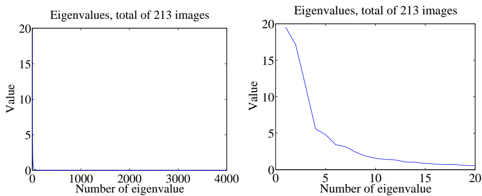
FIGURE 4.7: On the left , the eigenvalues of the covariance of the Japanese facial expression dataset; there are 4096, so it’s hard to see the curve (which is packed to the left). On the right , a zoomed version of the curve, showing how quickly the values of the eigenvalues get small.
