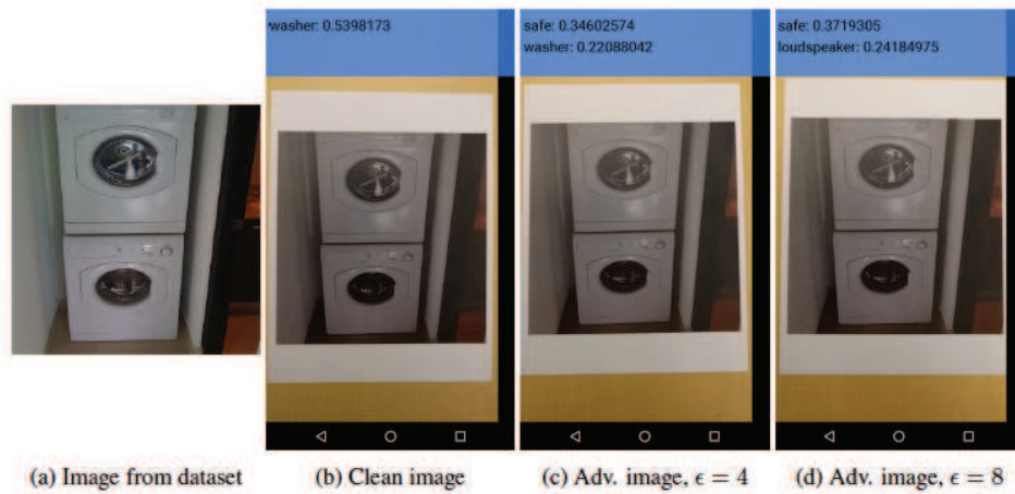
FIGURE 15.17: This figure is from “ADVERSARIAL EXAMPLES IN THE PHYSICAL WORLD”, by Alexey Kurakin et al.. The authors photographed the washing machine on the left. They then prepared clean and adversarial versions of that image and printed them. Finally, they photographed them with a cell-phone camera, producing the images with overprinting. The first is a photo of the printed washing machine, and is correctly classified as a washer ; the second and third are photos of printed adversarial examples, and are (respectively) a safe (or perhaps a washer ) and a safe (or perhaps a loudspeaker ).
