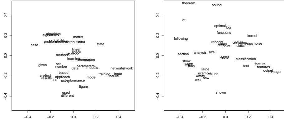
FIGURE 5.6: On the left , the 40 most frequent words in the NIPS dataset, plotted using a multidimensional scaling of the document frequencies, smoothed using latent semantic analysis. On the right , the next 40 most frequent words, plotted in the same way. I used 1000 dimensions for the smoothing. Words that have a similar pattern of incidence in documents appear near one another.
