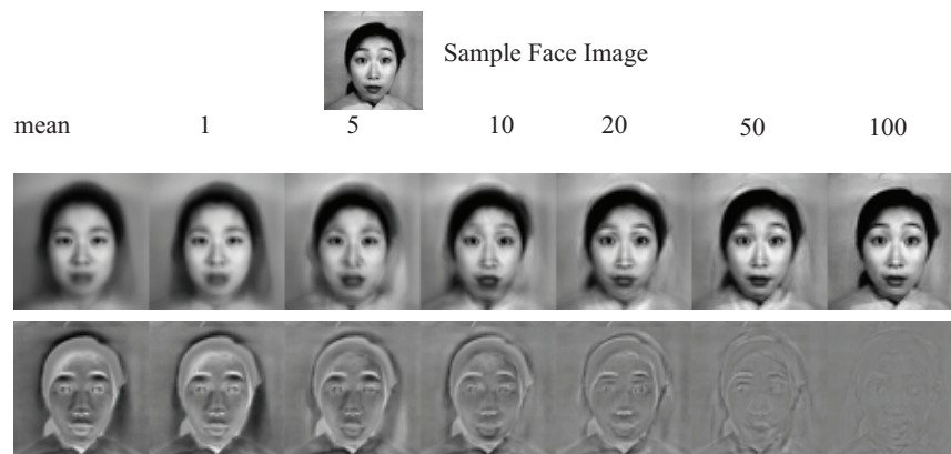
FIGURE 4.9: Approximating a face image by the mean and some principal components; notice how good the approximation becomes with relatively few components.
