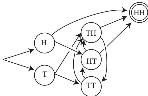
FIGURE 11.3: A directed graph representing the coin flip example, using the pairs of random variables described in worked example 11.3. A sequence “HTHTHH” (where the last two H’s are the last two flips) would be generated by transitioning to H, then to HT, then to TH, then to HT, then to TH, then to HH. By convention, the end state is a double circle. Each edge has probability 1/2 .
