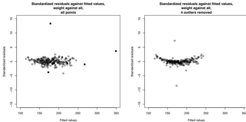
FIGURE 9.15: On the left, standardized residuals plotted against predicted value for weight regressed against all variables for the bodyfat dataset. Four data points appear suspicious, and I have marked these with a filled in marker. On the right, standardized residuals plotted against predicted value for weight regressed against all variables for the bodyfat dataset, but with the four suspicious looking data points removed. Notice two other points stick out markedly.
