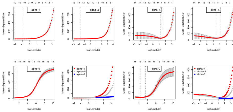
FIGURE 10.7: Plots of mean-squared error as a function of log regularization parameter (i.e. \log \lambda ) for a regression of weight against all variables for the bodyfat dataset using an elastic net regularizer for various choices of \alpha . The case \alpha = 1 corresponds to a lasso; \alpha = 0 corresponds to a ridge; and \alpha = 0.5 is one possible choice yielding an elastic net. These plots show mean-squared error averaged over cross-validation folds with a vertical one standard deviation bar. On the left , the plot for the dataset with the six outliers identified in Figure 287 removed. On the right , the plot for the whole dataset. Notice how the outliers increase the variability of the error, and the best error. The top row of numbers gives the number of non-zero components in \hat{\beta} . Notice how as \lambda increases, this number falls (there are 15 explanatory variables, so the largest model would have 15 variables). The penalty ensures that explanatory variables with small coefficients are dropped as \lambda gets bigger.
