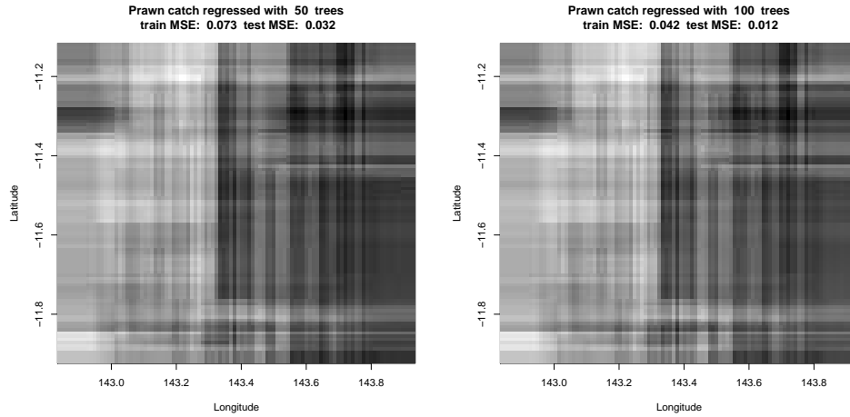
FIGURE 17.3: Score 1 of the prawn trawls data from http://www.statsci.org/data/oz/reef.html , regressed against latitude and longitude (I did not use depth, also in that dataset; this means I could plot the regression easily). The smallest value in the data is full dark; and the largest value is full light. The figure shows results of a greedy stagewise regression using regression trees using 50 and 100 trees. Notice that both train and test error go down, and the model gets more complex as we add trees.
