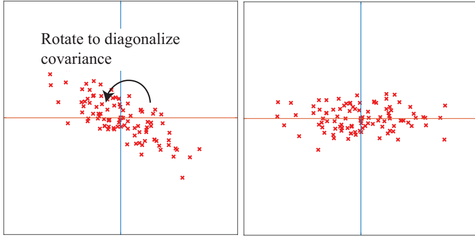
FIGURE 3.6: On the left , the translated blob of figure 3.5. This blob lies somewhat diagonally, because the vertical and horizontal components are correlated. On the right , that blob of data rotated so that there is no correlation between these components. We can now describe the blob by the vertical and horizontal variances alone, as long as we do so in the new coordinate system. In this coordinate system, the vertical variance is significantly larger than the horizontal variance — the blob is short and wide.
