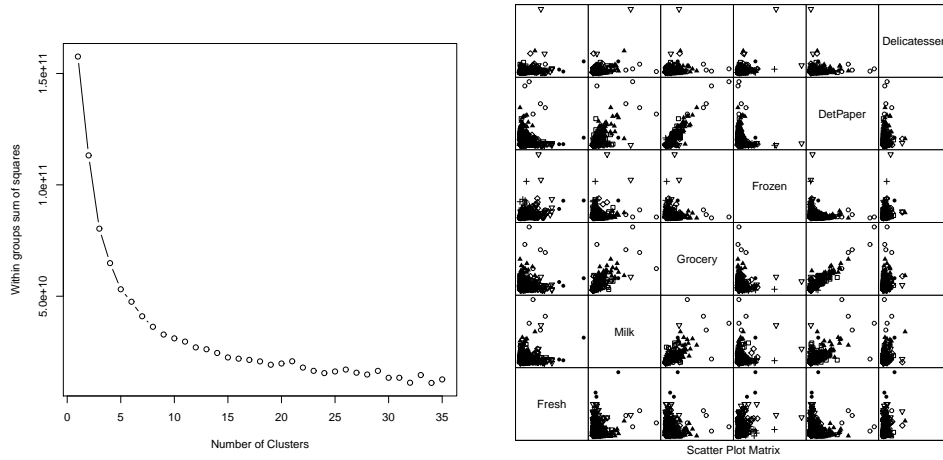
FIGURE 7.10: On the left , the cost function (of section 7.2) for clusterings of the customer data with k -means for k running from 2 to 35. This suggests using a k somewhere in the range 10-30; I chose 10. On the right , I have clustered this data to 10 cluster centers with k -means. The clusters do seem to be squashed together, but the plot on the left suggests that clusters do capture some important information. Using too few clusters will clearly lead to problems. Notice that I did not scale the data, because each of the measurements is in a comparable unit. For example, it wouldn't make sense to scale expenditures on fresh and expenditures on grocery with a different scale.
