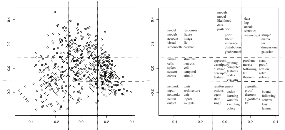
FIGURE 5.4: On the left, a multidimensional scaling mapping the NIPS documents into 2D. The distances between points represent (as well as an MDS can) the distances between normalized smoothed word counts. I have plotted every 10'th document, to avoid crowding the plot. Superimposed on the figure is a grid, dividing each coordinate at the 33% (resp. 66%) quantile. On the right, I have plotted the 10 words most strongly correlated with a document appearing in the corresponding grid block (highest correlation at top left in block, lowest in bottom right). Each block has quite different sets of words, but there is evidence that: changes in the coordinates result in changes in document content; the dataset still has proper names in it, though insiders might notice the names are in sensible places; the horizontal coordinate seems to represent a practical-conceptual axis; and increasing values of the vertical coordinate seems to represent an increasingly statistical flavor. This is (rather rough) evidence that distances between smoothed normalized word counts do capture aspects of meaning.
