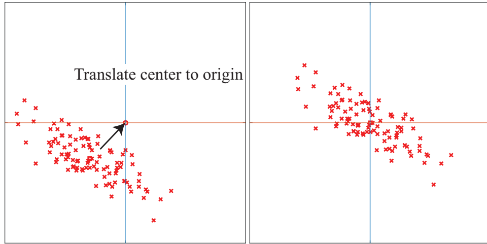
FIGURE 3.5: On the left , a “blob” in two dimensions. This is a set of data points that lie somewhat clustered around a single center, given by the mean. I have plotted the mean of these data points with a hollow square (it’s easier to see when there is a lot of data). To translate the blob to the origin, we just subtract the mean from each datapoint, yielding the blob on the right .
