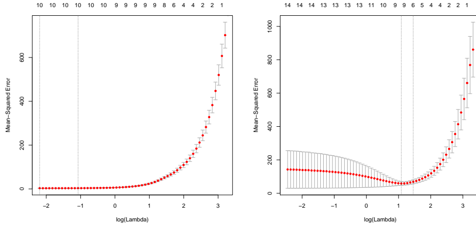
FIGURE 10.4: Plots of mean-squared error as a function of log regularization parameter (i.e. \log \lambda ) for a regression of weight against all variables for the bodyfat dataset using an L1 regularizer (i.e. a lasso). These plots show mean-squared error averaged over cross-validation folds with a vertical one standard deviation bar. On the left , the plot for the dataset with the six outliers identified in Figure 287 removed. On the right , the plot for the whole dataset. Notice how the outliers increase the variability of the error, and the best error. The top row of numbers gives the number of non-zero components in \hat{\beta} . Notice how as \lambda increases, this number falls (there are 15 explanatory variables, so the largest model would have 15 variables). The penalty ensures that explanatory variables with small coefficients are dropped as \lambda gets bigger.
