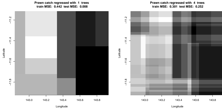
FIGURE 17.2: Score 1 of the prawn trawls data from http://www.statsci.org/data/oz/reef.html , regressed against latitude and longitude (I did not use depth, also in that dataset; this means I could plot the regression easily). The smallest value in the data is full dark; and the largest value is full light. The figure shows results of a greedy stagewise regression using regression trees using 1 and 4 trees. The figure on the left is different from the tree of figure 17.1 because I used a test-train split in this case, and different settings for rpart . Notice that both train and test error go down, and the model gets more complex as we add trees. Further stages appear in figure 17.3, which uses the same intensity scale.
