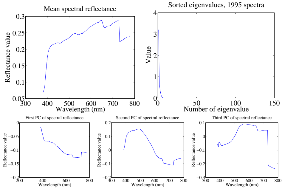
FIGURE 4.5: On the top left , the mean spectral reflectance of a dataset of 1995 spectral reflectances, collected by Kobus Barnard (at http://www.cs.sfu.ca/~colour/data/ ). On the top right , eigenvalues of the covariance matrix of spectral reflectance data, from a dataset of 1995 spectral reflectances, collected by Kobus Barnard (at http://www.cs.sfu.ca/~colour/data/ ). Notice how the first few eigenvalues are large, but most are very small; this suggests that a good representation using few principal components is available. The bottom row shows the first three principal components. A linear combination of these, with appropriate weights, added to the mean ( top left ), gives a good representation of the dataset.
