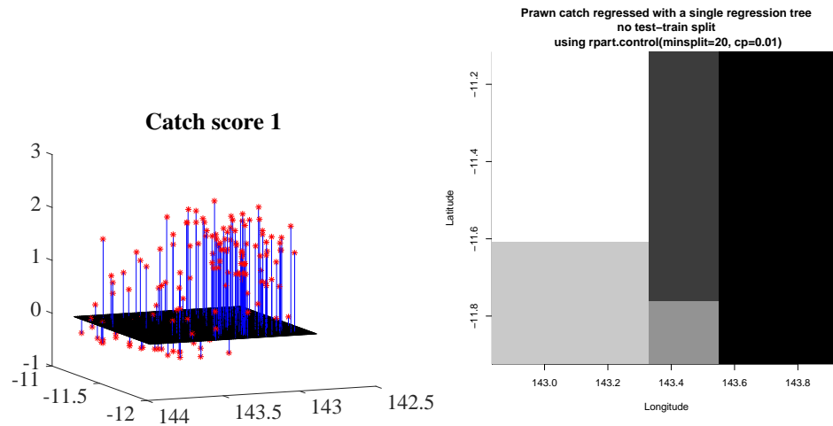
FIGURE 17.1: On the left , a 3D scatter plot of score 1 of the prawn trawls data from http://www.statsci.org/data/oz/reef.html , plotted as a function of latitude and longitude. On the right , a regression using a single regression tree, to help visualize the kind of predictor these trees produce. You can see what the tree does: carve space into boxes, then predict a constant inside each.
