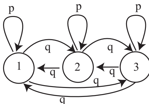
FIGURE 11.4: A virus can exist in one of 3 strains. At the end of each year, the virus mutates. With probability \alpha , it chooses uniformly and at random from one of the 2 other strains, and turns into that; with probability 1 - \alpha , it stays in the strain it is in. For this figure, we have transition probabilities p = (1 - \alpha) and q = (\alpha/2) .
