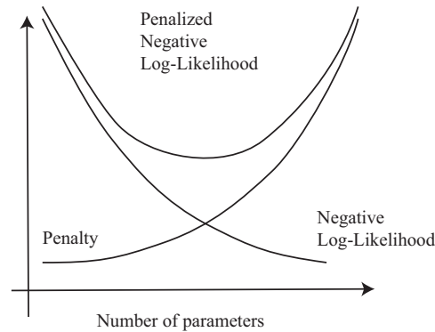
FIGURE 10.1: When we add explanatory variables (and so parameters) to a model, the value of the negative log-likelihood of the best model can't go up, and usually goes down. This means that we cannot use the value as a guide to how many explanatory variables there should be. Instead, we add a penalty that increases as a function of the number of parameters, and search for the model that minimizes the sum of negative log-likelihood and penalty. AIC and BIC grow linearly with the number of parameters, but I am following the usual convention of plotting the penalty as a curve rather than a straight line.
