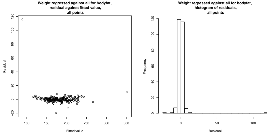
FIGURE 10.3: A robust linear regression of weight against all variables for the bodyfat dataset, using the Huber loss and all data points. On the left , residual plotted against fitted value (the residual is not standardized). Notice that there are some points with very large residual, but most have much smaller residual; this wouldn't happen with a squared error. On the right , a histogram of the residual. If one ignores the extreme residual values, this looks normal. The robust process has been able to discount the effect of the outliers, without us needing to identify and reject outliers by hand.
