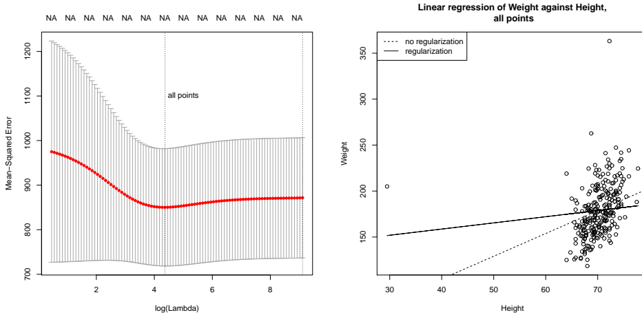
FIGURE 9.13: Regularization doesn't make outliers go away. On the left, cross-validated error estimated for different choices of regularization constant for a linear regression of weight against height for the bodyfat dataset, with all points. The horizontal axis is log regression constant; the vertical is cross-validated error. The mean of the error is shown as a spot, with vertical error bars. The vertical lines show a range of reasonable choices of regularization constant (left yields the lowest observed error, right the error whose mean is within one standard error of the minimum). On the right, two regression lines on a scatter plot of this dataset; one is the line computed without regularization, the other is obtained using the regularization parameter that yields the lowest observed error. In this case, the regularizer doesn't change the line much, but may produce improved values on new data (notice how the cross-validated error is fairly flat with low values of the regularization constant).
