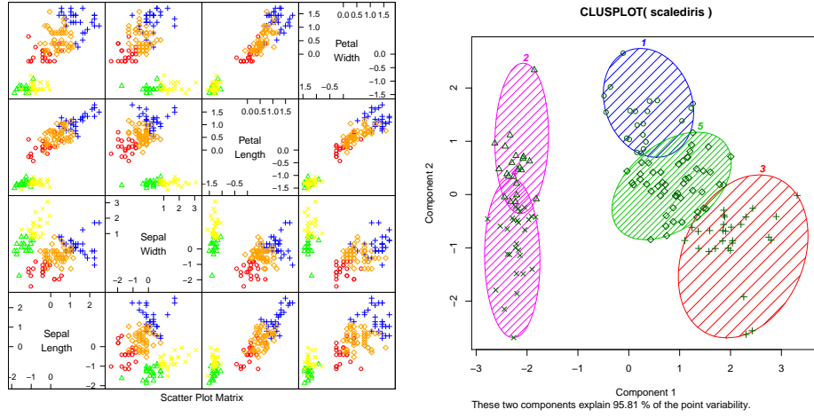
FIGURE 7.7: On the left , a panel plot of the iris data clustered using k -means with k = 5 . By comparison with figure 7.8, notice how setosa seems to have been broken in two groups, and versicolor and virginica into a total of three. On the right , this data set projected onto the first two principal components, with one blob drawn over each cluster.
