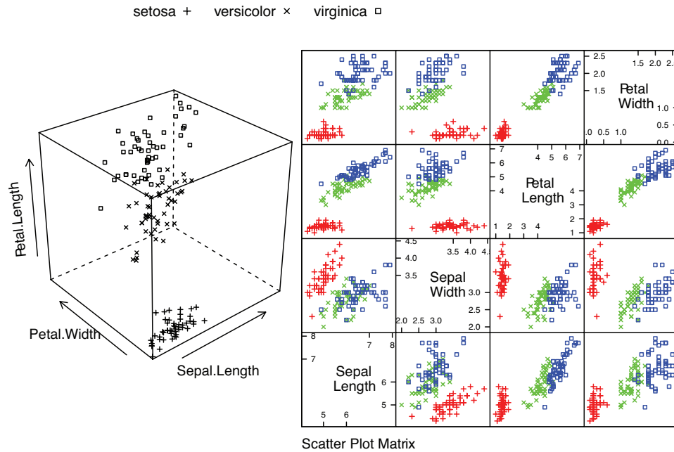
FIGURE 3.3: Left: the 3D scatterplot of the iris data of Figure 3.1, for comparison. Right: a scatterplot matrix for the Iris data. There are four variables, measured for each of three species of iris. I have plotted each species with a different marker. You can see from the plot that the species cluster quite tightly, and are different from one another.
