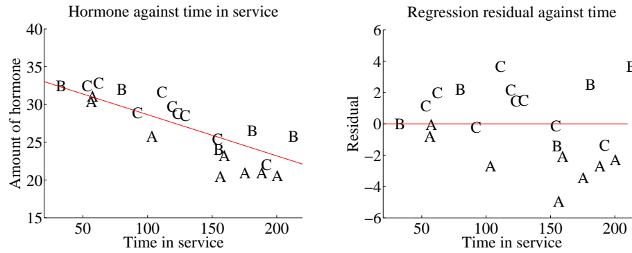
FIGURE 9.3: On the left , a scatter plot of hormone against time for devices from tables 9.1 and 9.1. Notice that there is a pretty clear relationship between time and amount of hormone (the longer the device has been in service the less hormone there is). The issue now is to understand that relationship so that we can tell whether lots A, B and C are the same or different. The best fit line to all the data is shown as well, fitted using the methods of section 9.2. On the right , a scatter plot of residual — the distance between each data point and the best fit line — against time for the devices from tables 9.1 and 9.1. Now you should notice a clear difference; some devices from lots B and C have positive and some negative residuals, but all lot A devices have negative residuals. This means that, when we account for loss of hormone over time, lot A devices still have less hormone in them. This is pretty good evidence that there is a problem with this lot.
