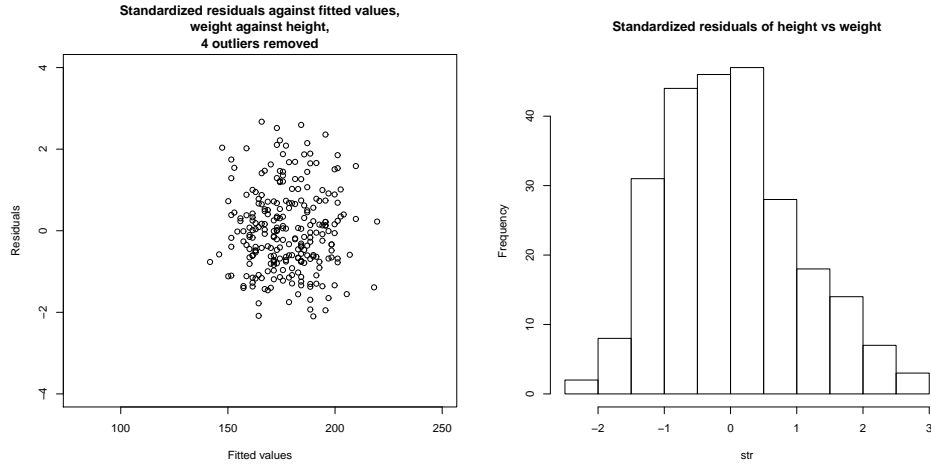
FIGURE 9.9: On the left , standardized residuals plotted against predicted value for weight regressed against height for the bodyfat dataset. I removed the four suspicious looking data points, identified in Figure 9.7 with filled-in markers ; these seemed the most likely to be outliers. You should compare this plot with the residuals in figure 9.8, which are not standardized. On the right , a histogram of the residual values. Notice this looks rather like a histogram of a standard normal random variable, though there are slightly more large positive residuals than one would like. This suggests the regression is working tolerably.
