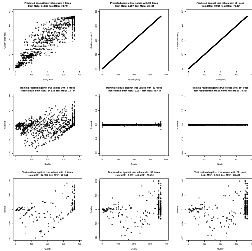
FIGURE 17.4: Diagnostic data from a stagewise regression of rank of quality of education against all other variables except overall rank and name for the data of https://www.kaggle.com/mylesoneill/world-university-rankings/data . Top row: Model predictions against true values; middle row: residual against true values, training examples; bottom row: residuals against true values, test examples. Details in the worked example.
