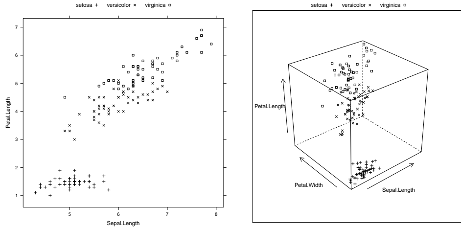
FIGURE 3.1: Left: a 2D scatterplot for the famous Iris data. I have chosen two variables from the four, and have plotted each species with a different marker. Right: a 3D scatterplot for the same data. You can see from the plots that the species cluster quite tightly, and are different from one another. If you compare the two plots, you can see how suppressing a variable leads to a loss of structure. Notice that, on the left, some 'x's lie on top of boxes; you can see that this is an effect of projection by looking at the 3D picture (for each of these data points, the petal widths are quite different). You should worry that leaving out the last variable might have suppressed something important like this.
