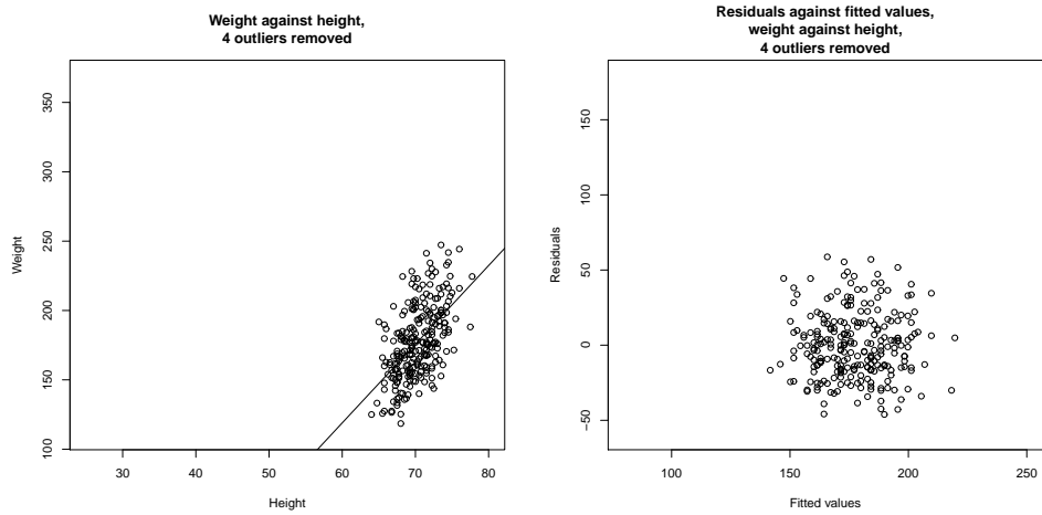
FIGURE 9.8: On the left , weight regressed against height for the bodyfat dataset. I have now removed the four suspicious looking data points, identified in Figure 9.7 with filled-in markers; these seemed the most likely to be outliers. On the right , a scatter plot of the residual against the value predicted by the regression. Notice that the residual looks like noise. The residual seems to be uncorrelated to the predicted value; the mean of the residual seems to be zero; and the variance of the residual doesn't depend on the predicted value. All these are good signs, consistent with our model, and suggest the regression will yield good predictions.
