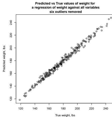
FIGURE 9.18: A scatter plot of the predicted weight against the true weight for the bodyfat dataset. The prediction is made with all variables, but the six outliers identified above are omitted. I used a Box-Cox transformation with parameter 1/2 , and the regularization parameter that yielded the smallest mean square error in Figure 9.17.
