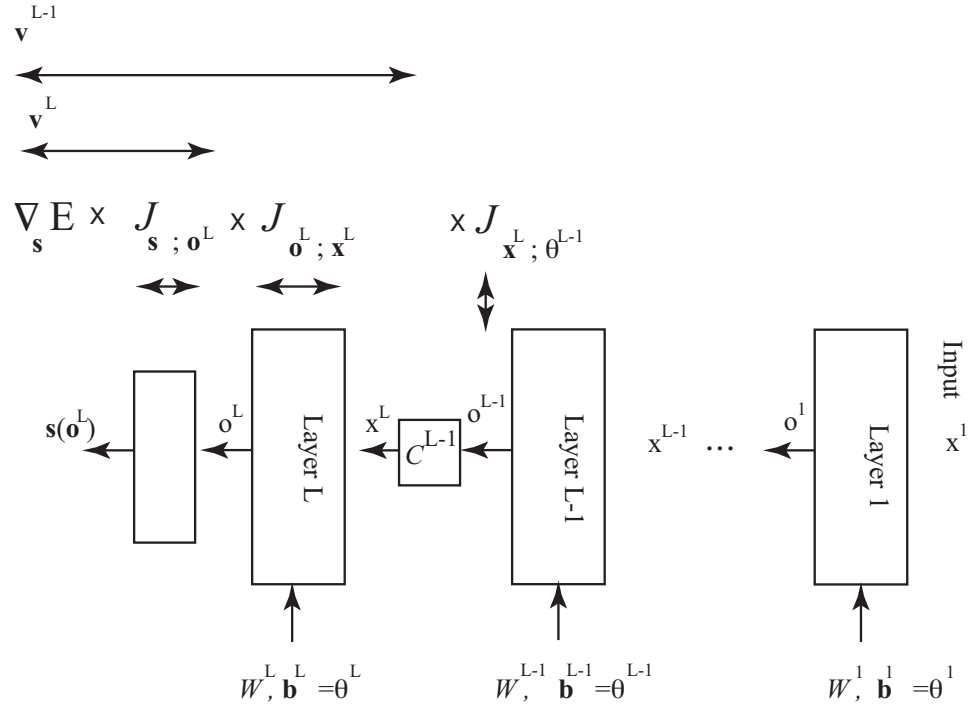
FIGURE 15.5: Constructing the gradient with respect to \theta^{L-1} .
