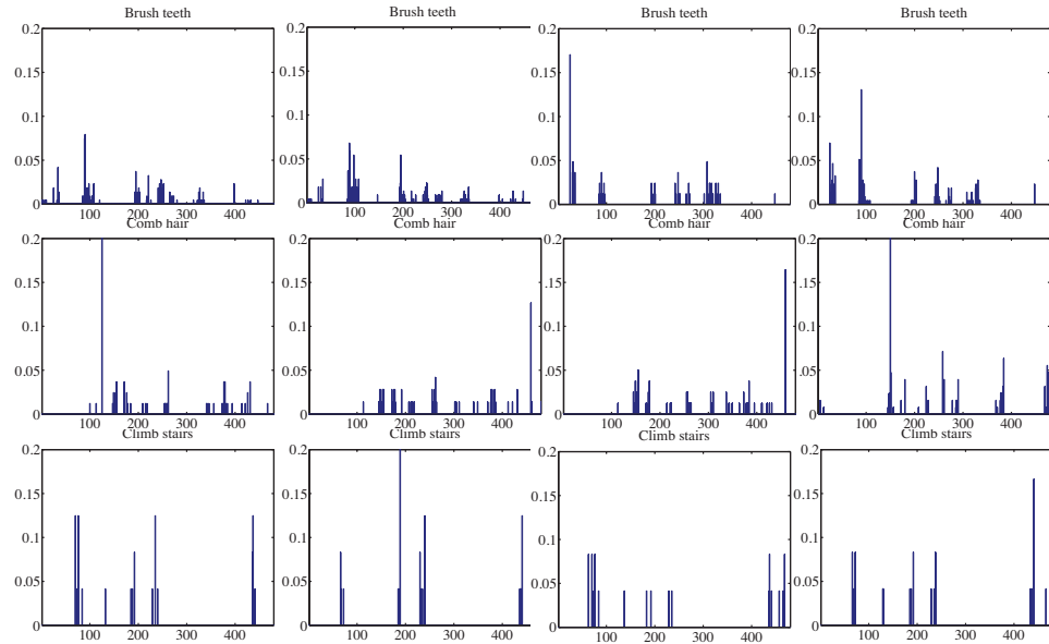
FIGURE 7.15: Histograms of cluster centers for the accelerometer dataset, for different activities. You should notice that (a) these histograms look somewhat similar for different actors performing the same activity and (b) these histograms look somewhat different for different activities.
