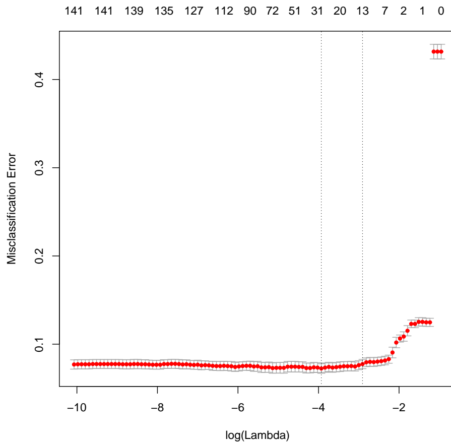
FIGURE 21.8: A cross-validation plot from cv.glmnet for the lasso applied to predictions on test data obtained from all 150 trees from the boosting of figure 21.7. Quite small models do rather well, and somewhere between 13 and 30 predictors looks like the best. However, one needs to be careful how one chooses a model.
