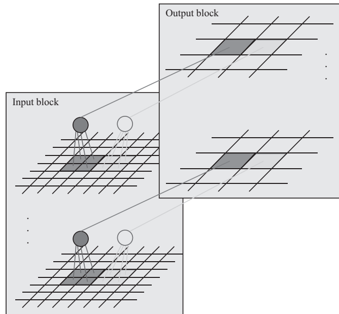
FIGURE 18.2: In a pooling layer, pooling units compute the largest value of their inputs, then pass it on. The most common case is 2 \times 2 , illustrated here. We tile each slice with 2 \times 2 windows that do not overlap. Pooling units compute the max, then pass that on to the corresponding location in the corresponding slice of the output block. As a result, the spatial dimensions of the output block will be about half those of the input block (details depend on how one handles windows that hang over the edge).
