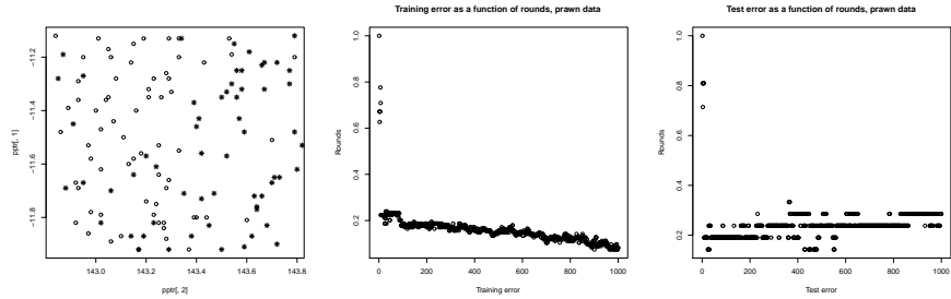
FIGURE 21.5: On the left, a scatter plot of the prawn data. The circles are locations where the prawn catch exceeded the median; the stars are locations where the catch was below median. Center shows the training error for a boosted classifier using decision stumps, as a function of the number of stumps. Notice how adding a stump causes the training error to fall slowly but reliably even when we already have many predictors. Right shows the test error, which settles close to a fixed value fairly quickly. This isn't typical behavior – it is common to observe the test error falling reliably as well. Figure ?? visualizes the predictors.
