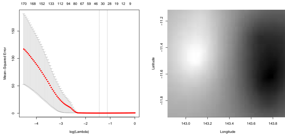
FIGURE 13.9: The prawn data of figure 13.6, now smoothed with glmnet. On the left, the plot of held out error vs log regularization weight produced by glmnet for the prawn data, as described in example 13.1. Notice that the best regression uses between 20 and 30 of 930 possible features. On the right, a heat map. case, a Gaussian kernel) with scale chosen by cross-validation.
