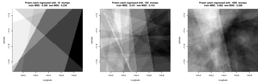
FIGURE 21.6: Visualizations of the predictor for the prawn data of worked example 21.4. Mid-grey is zero; white is positive (and so any shade in the range mid-grey to white predicts a score greater than the median); black is negative (and so any shade in the range mid-grey to black predicts a score less than the median). The predictor formed by one stump cuts the region into two halves with a line; on one side of the line, it takes one constant value, and on the other, it takes a different constant value. Adding many of these together results in a function that is constant in each cell of an arrangement of lines. Predictors that use more stumps produce more complicated functions of this form, with improvements in training error and some improvement in test error (Figure 21.6).
