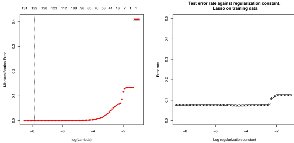
FIGURE 21.9: Left: A cross-validation plot from cv.glmnet for the lasso applied to predictions on training data obtained from all 150 trees from the boosted model of Figure 21.7. Notice that this suggests zero error is attainable by quite small models. But the cross-validated error here is biased low, because the predictors were trained on all the data, so they have seen data on the test side of each test-train split. Right: The test error of the best model for each value of the regularization constant in the plot on the left. Notice how cross-validating on the training set has biased the estimate low – you won’t in practice get zero error.
