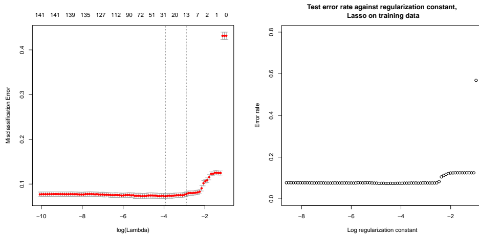
FIGURE 21.10: Left: A cross-validation plot from cv.glmnet for the lasso applied to predictions on test data passed through each of the 150 trees made by the boosted model of Figure 21.7. This gives a much better estimate of the error, as you can see by comparing to the test error of the best model for each value of the regularization constant ( right ). This approach gives a better estimate of what the model will do, but may present problems if you have little data.
