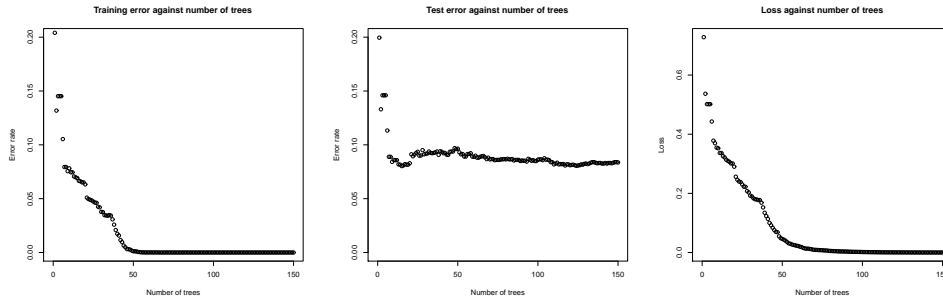
FIGURE 21.7: Models for a boosted decision tree classifier predicting whether a given prescriber will write more than 10 opioid prescriptions in a year, using the data of https://www.kaggle.com/apryor6/us-opiate-prescriptions . Left: training error against number of trees; center: test error against number of trees; right: exponential loss against number of trees. Notice that both test and train error go down, but there is a test-train gap. Notice also a characteristic property of boosting; continuing to boost after the training error is zero (about 50 trees in this case) still results in improvements in the test error. Note also that lower exponential loss doesn't guarantee lower training error.
