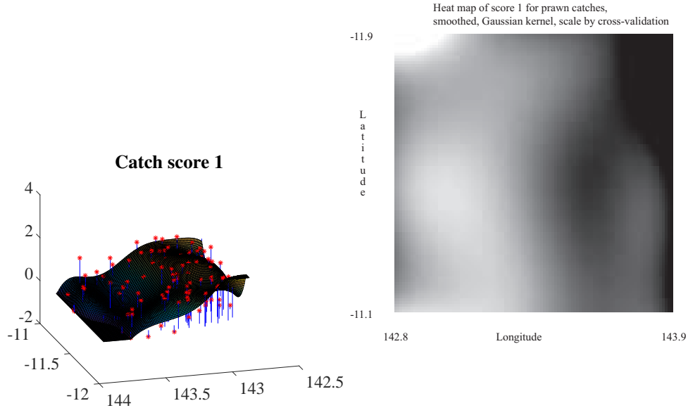
FIGURE 13.7: The prawn data of figure 13.6, smoothed with radial basis functions (in this case, a Gaussian kernel) with scale chosen by cross-validation. On the left, a surface shown with the 3D scatter plot. On the right, a heat map. I ignored the curvature of the earth, small at this scale, when computing distances between points. I used 60 basepoints, constructed by choosing 60 of 155 training points at random, then adding a small random offset.
