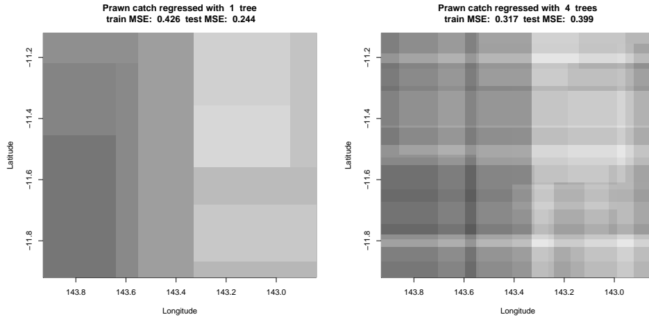
FIGURE 21.2: Score 1 of the prawn trawls data from http://www.statsci.org/data/oz/reef.html , regressed against latitude and longitude (I did not use depth, also in that dataset; this means I could plot the regression easily). The axes (horizontal runs from bigger to smaller) are chosen so that you can register with the plot in figure 21.1 by eye. The intensity scale is chosen so that the range is symmetric; because there are no small negative numbers, there are no very dark boxes. The figure shows results using 1 and 4 trees. The figure on the left is slightly different from the tree of figure 21.1 because I used a test-train split in this case, and different settings for rpart . Notice the model gets more complex as we add trees. Further stages appear in figure 21.3, which uses the same intensity scale.
