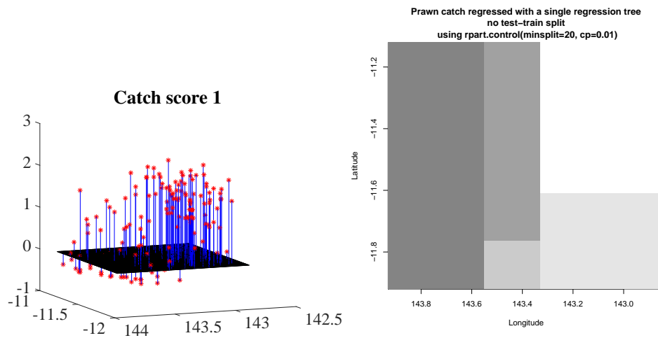
FIGURE 21.1: On the left, a 3D scatter plot of score 1 of the prawn trawls data from http://www.statsci.org/data/oz/reef.html , plotted as a function of latitude and longitude. On the right, a regression using a single regression tree, to help visualize the kind of predictor these trees produce. You can see what the tree does: carve space into boxes, then predict a constant inside each. The intensity scale is chosen so that the range is symmetric; because there are no small negative numbers, there are no very dark boxes. The odd axes (horizontal runs from bigger to smaller) are chosen so that you can register the left to the right by eye.
