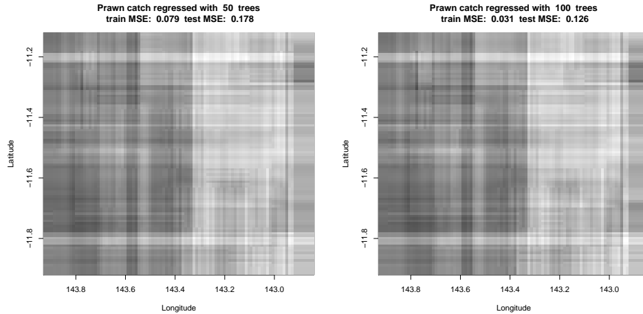
FIGURE 21.3: Score 1 of the prawn trawls data from http://www.statsci.org/data/oz/reef.html , regressed against latitude and longitude (I did not use depth, also in that dataset; this means I could plot the regression easily). The axes (horizontal runs from bigger to smaller) are chosen so that you can register with the plot in figure 21.1 by eye. The intensity scale is chosen so that the range is symmetric; because there are no small negative numbers, there are no very dark boxes. The figure shows results of a greedy stagewise regression using regression trees using 50 and 100 trees. Notice that both train and test error go down, and the model gets more complex as we add trees.
