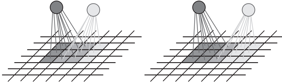
FIGURE 18.1: Figure 17.9 shows units taking an input block and creating an output block. Each unit is fed by a window on the spatial dimensions of the input block. The window is advanced by the stride to feed the next unit. On the left , two units fed by 3 \times 3 windows with a stride of 1. I have shaded the pixels in the window to show which pixels go to which unit; notice the units share 6 pixels. In this case, the spatial dimensions of the output block will be either the same as those of the input block (if we find some values to feed pixels in windows that hang over the edge of the image), or only slightly smaller (if we ignore units whose windows hang over the edges of the image). On the right , two units fed by 3 \times 3 windows with a stride of 2. Notice the units share fewer pixels, and the output block will be smaller than the input block.
