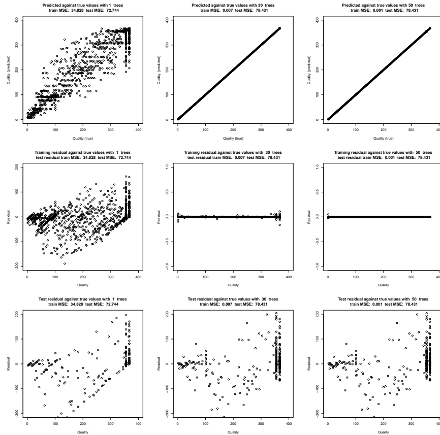
FIGURE 21.4: Diagnostic data from a stagewise regression of rank of quality of education against all other variables except overall rank and name for the data of https://www.kaggle.com/mylesoneill/world-university-rankings/data . Top row: Model predictions against true values; middle row: residual against true values, training examples; bottom row: residuals against true values, test examples. Details in the worked example.
