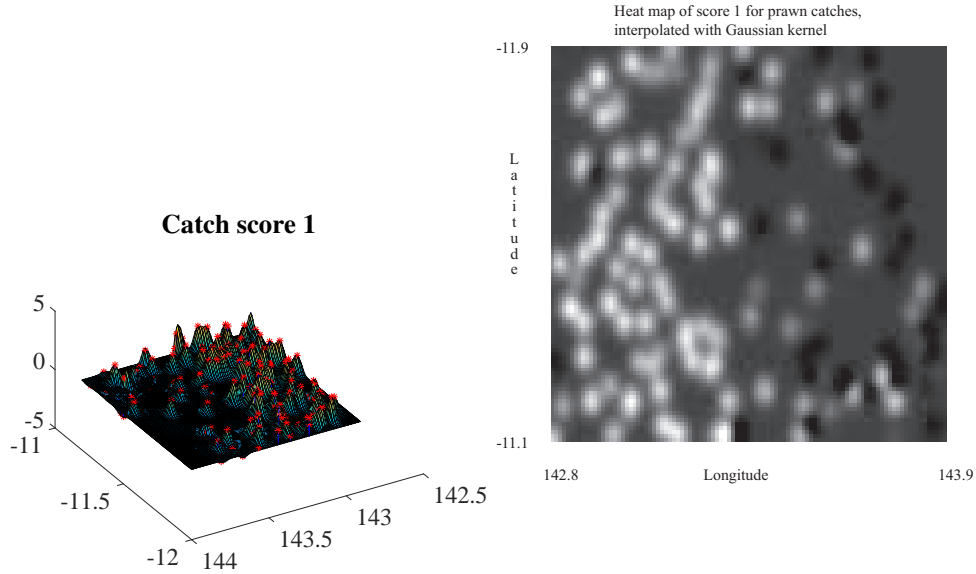
FIGURE 13.8: The prawn data of figure 13.6, interpolated with radial basis functions (in this case, a Gaussian kernel) with scale chosen by cross-validation. On the left, a surface shown with the 3D scatter plot. On the right, a heat map. I ignored the curvature of the earth, small at this scale, when computing distances between points. This figure is a good example of why interpolation is usually not what one wants to do (text).
