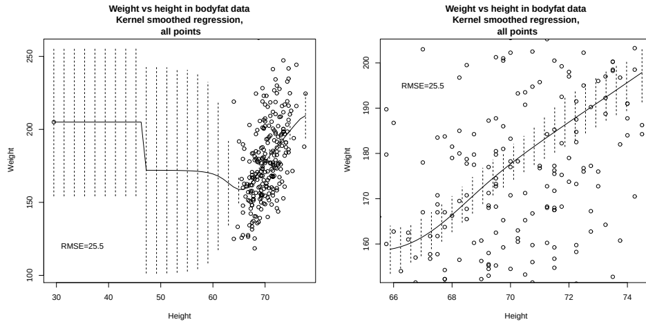
FIGURE 13.4: A non-parametric regression, using kernel smoothing, of weight against height, using the dataset of Figure 56. On the left , a curve showing the expected value of the independent variable for each value of the explanatory variable, with axes chosen to show the outlying point. The vertical bars show the standard error of the predicted density for the independent variable, for each value of the explanatory variable. Notice the method can make predictions around this point, but that these predictions have very large standard error as one would expect. On the right , the same curve, but on axes chosen to display the non-outlying points. The bars are small, because the standard error is small here (this isn't the same as the standard deviation of the predictive distribution).
