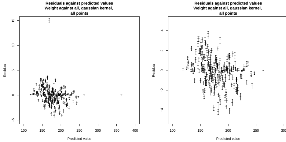
FIGURE 13.5: A non-parametric regression, using kernel smoothing, of weight against all variables, using the bodyfat dataset of Figure 56. On the left , a scatterplot of the predicted value against residual, on axes that show all points. The residual has not been standardized, because it is unclear how to do so. I have shown a one standard error bar for the residual as a vertical bar, plotted at the mean predicted value. For some points, the standard error is very small, so you can only see a horizontal bar. Notice how some points have a large residual, but most residuals are in a reasonable range. On the right , the same plot, but on axes chosen to display the non-outlying points. The bars are small, because the standard error is small here (this isn't the same as the standard deviation of the predictive distribution).
