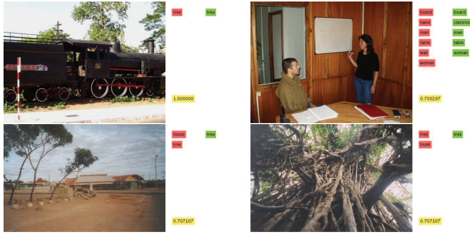
FIGURE 8.2: Four images with true (in red) and predicted (green) label words. Words are predicted using a CCA of image features and word vectors, as described in the text. Images are from a test set, not used in constructing the CCA. The yellow box gives the cosine distance between the predicted and true word vectors, smoothed by projection to a 150 dimensional space as in section 56. For these images, the cosine distances are reasonably close to one, and the predictions are quite good.
