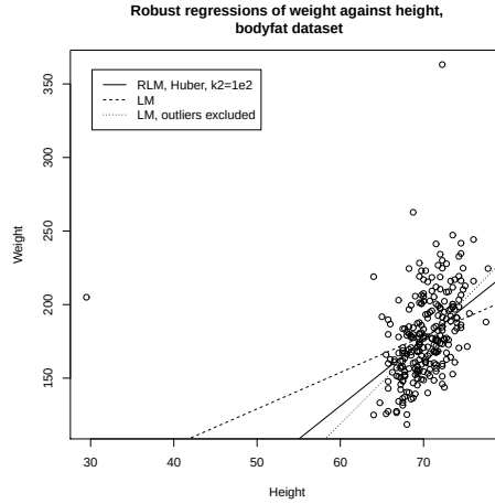
FIGURE 12.2: Comparing three different linear regression strategies on the bodyfat data, regressing weight against height. Notice that using an M -estimator gives an answer very like that obtained by rejecting outliers by hand. The answer may well be “better” because it isn’t certain that each of the four points rejected is an outlier, and the robust method may benefit from some of the information in these points. I tried a range of scales for the Huber loss (the ‘ k2 ’ parameter), but found no difference in the line resulting over scales varying by a factor of 1e4 , which is why I plot only one scale.
