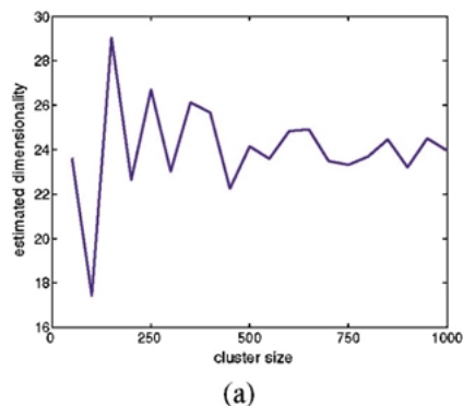
Figure 4. Convergence of d -estimate with cluster size, for synthesized polygons. (a) Estimated dimension converges to around d = 24 as cluster size increases to 1000 (true dimension d = 22 ). (b) Estimated dimensionality (solid) closely follows ground truth dimensionality (dashed). Dimension appears to be consistently slightly overestimated (cluster size N = 1000 ). This may be due to the approximation inherent in using the chamfer distance.
