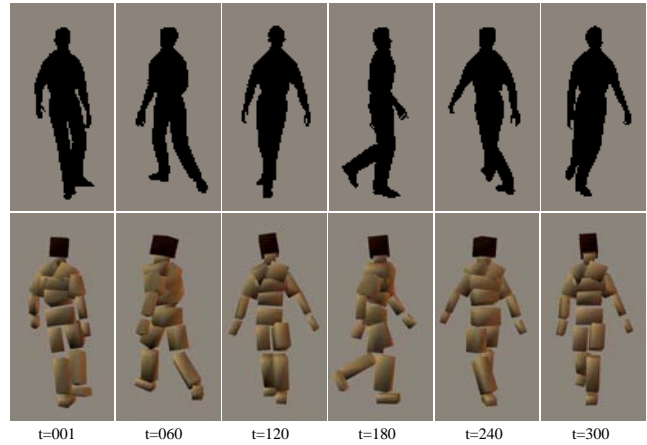
Figure 6. Some sample pose reconstructions for a spiral walking sequence not included in the training data, corresponding to figures 5(c) & (f). The reconstructions were computed with a Gaussian kernel RVM, using only 348 of the 1927 training examples. The average RMS estimation error per d.o.f. over the whole sequence is 4.1^\circ .
