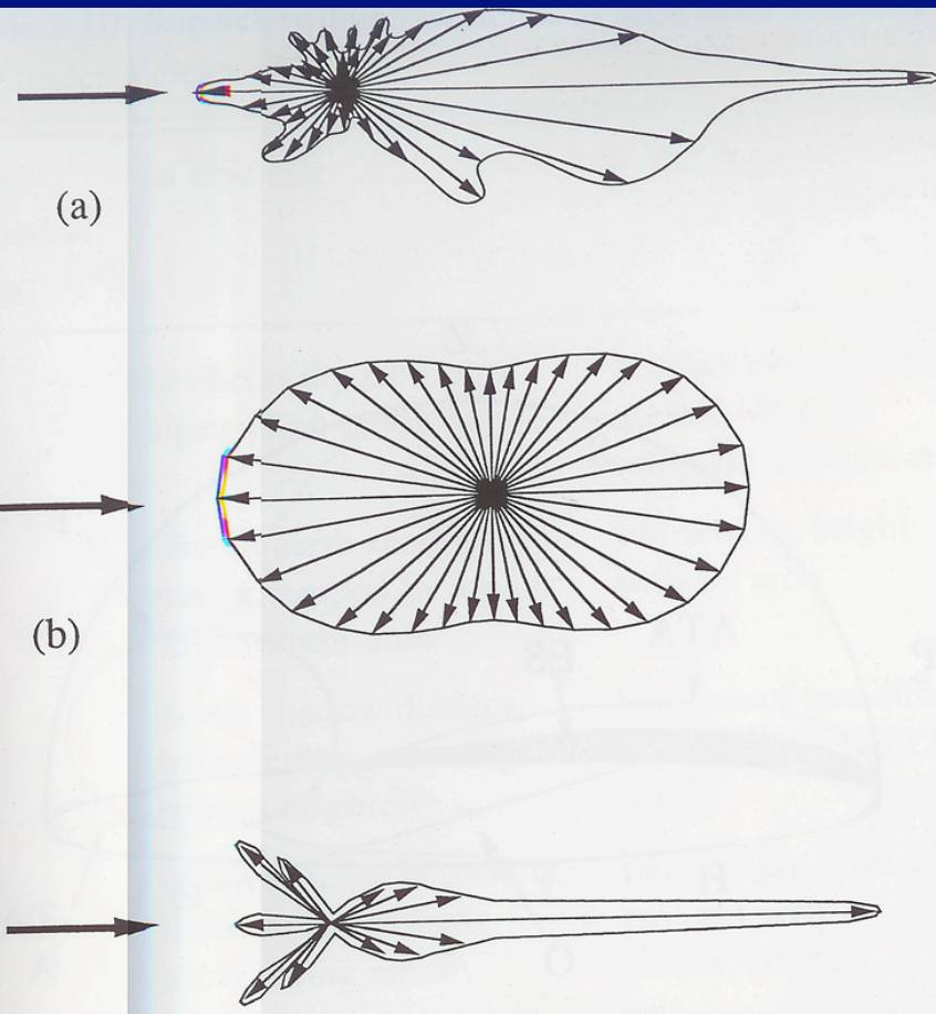
Fig. 2.7C Scattering patterns for different particles. (a) Large irregular particles, like those comprising dust and smoke, are irregular in the sense that they are not symmetric. They do, however, have a strong forward scattering peak and a smaller though still pronounced backscattering peak. (b) Air molecules have a scattering function that is symmetric fore and aft: they scatter the same amount of light in both the forward and backward directions but lack both the forward and backscattering peak. (c) Large water drops have a strong forward and backscattering peak and also show strong enhancements at the primary and secondary rainbow angles.
