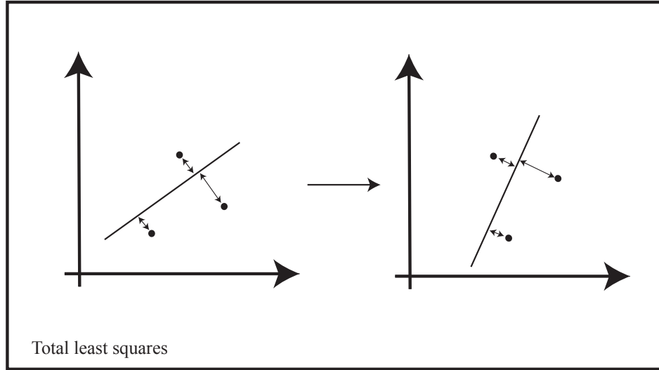
FIGURE 12.2: Total least-squares finds the line that minimizes the sum of squared perpendicular distances between tokens and the line so near-vertical lines can be fitted without difficulty. If the coordinate system rotates (say, the camera is rotated), the error between the rotated points and the rotated lines does not change.
