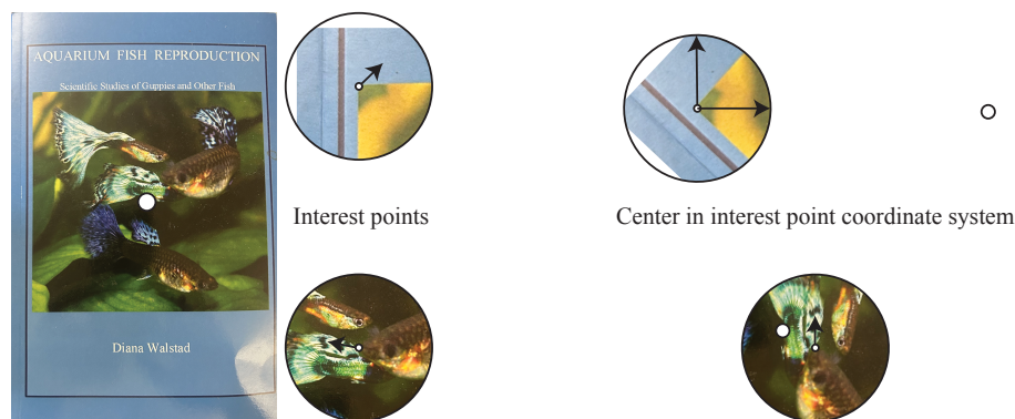
FIGURE 11.4: Interest points can vote on the location of the center of the book, because each interest point carries its own coordinate system. On the left , the cover image, with the center of the cover marked as an empty circle. Center shows two interest points, with their coordinate systems attached. I have marked the origin of the coordinate system with another circle, and the orientation with an arrow. On the right , I show each interest point rotated so that the coordinate systems line up, and mark the location of the center of the book in each point's coordinate system. For the top interest point, the book center is quite far away from the origin, but for the bottom interest point, it is quite close. Image credit: Cover of Diana Walstad's fascinating book on reproduction in aquarium fish, mostly guppies.
