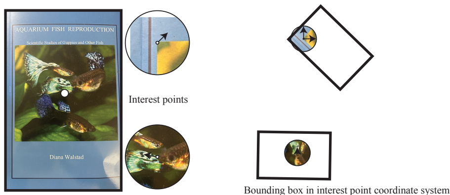
FIGURE 11.6: Interest points can vote on center location, orientation and scale of the book cover. This information yields the outline of the book, so you can think of interest points each carrying a vote as to the book cover outline. On the left , the cover image, with the outline marked in heavy lines. Center shows two interest points, with their coordinate systems attached. On the right , I show each interest point rotated so that the coordinate systems line up. I have marked the outline of the cover, in the interest point's coordinate system with heavy lines. Image credit: Cover of Diana Walstad's fascinating book on reproduction in aquarium fish, mostly guppies.
