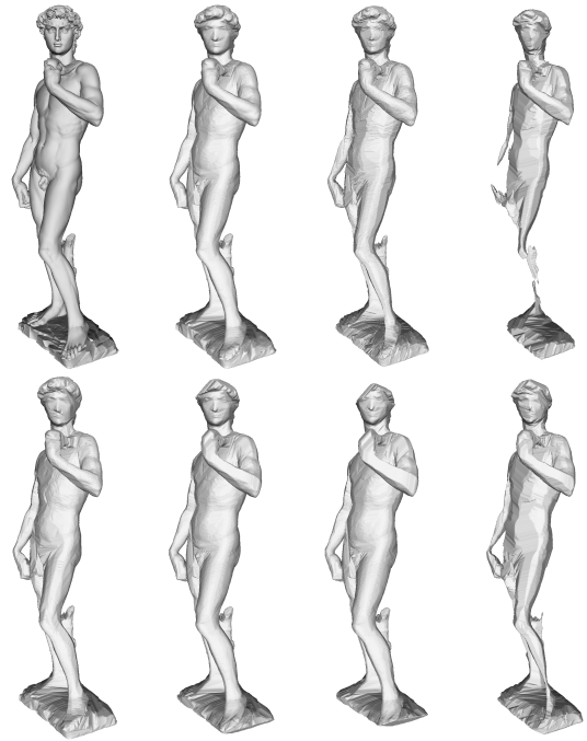
Figure 7: Performance of shape-from-silhouette reconstructions against various server defenses. Top row: original model, reconstruction from defenseless server, reconstruction with 0.5^\circ and 2.0^\circ perturbations of the view direction. Bottom row: reconstruction with a random image offset of 4 pixels, with 1.2% and 2.5% radial image distortion, and reconstruction against combined defenses ( 1.0^\circ view perturbation, 2 pixel random offset, and 1.2% radial image distortion).
