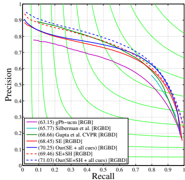
Fig. 3. Precision-recall curve on boundaries on the NYUD2 dataset.
