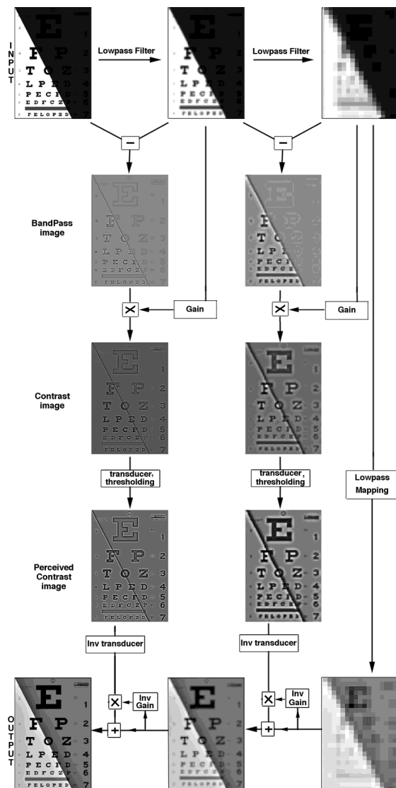
Figure 8: Pictorial representation of the computational model. Note that only 2 out of the 6 spatial mechanisms of one of the channels have been shown for the purpose of illustration. Original image is a Snellen chart with a 30:1 shadow boundary.
